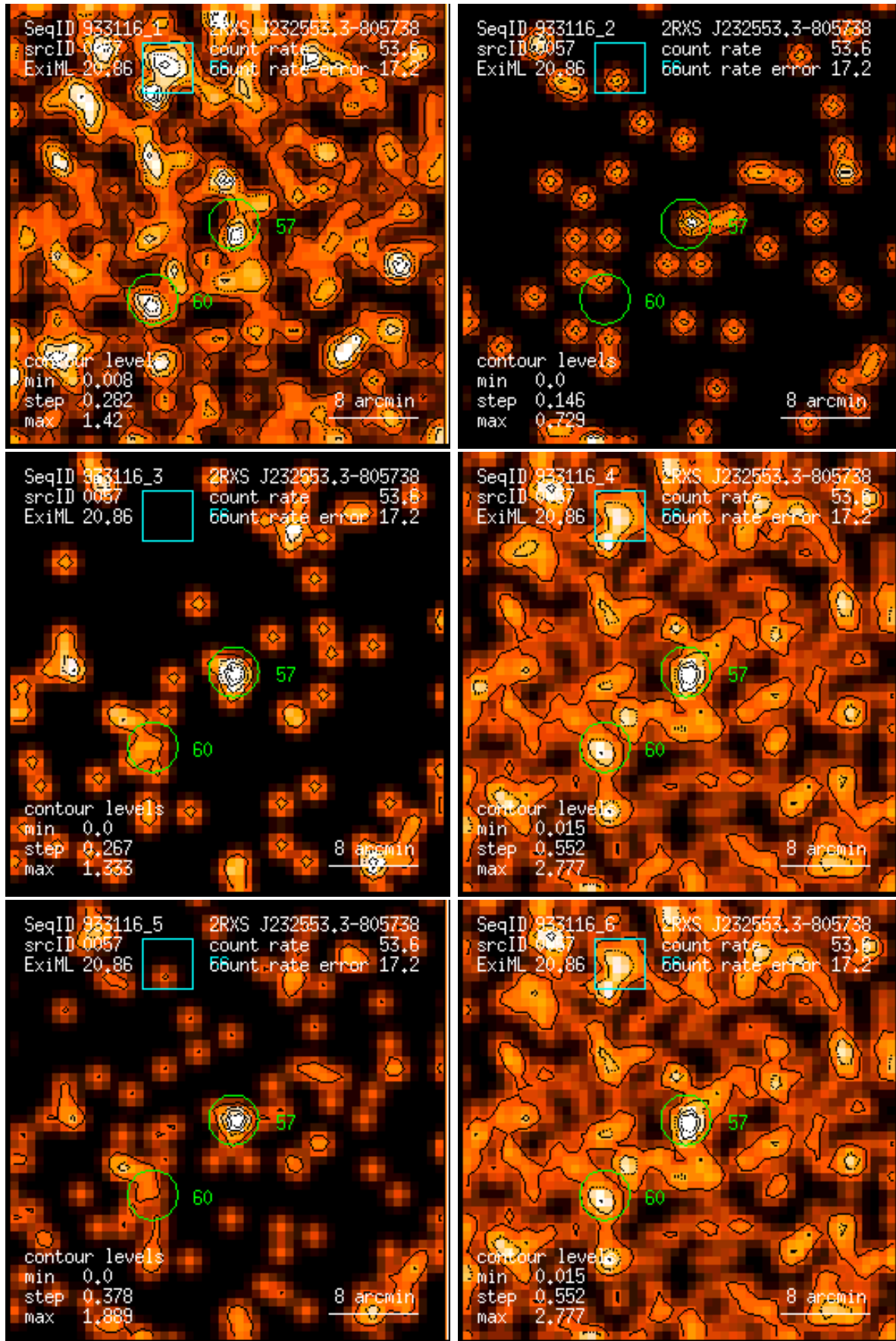
Figure 57: RASS 933116: detection 0057: band rate images, Gaussian filter: (1) PSPC channels 11 – 41, (2) 52 – 90, (3) 91 – 201, (4) 11 – 235, (5) 52 – 201, (6) 11 – 201. Broad band rates in counts/ks. Band rate contour levels in counts/ks/arcmin 2 .
