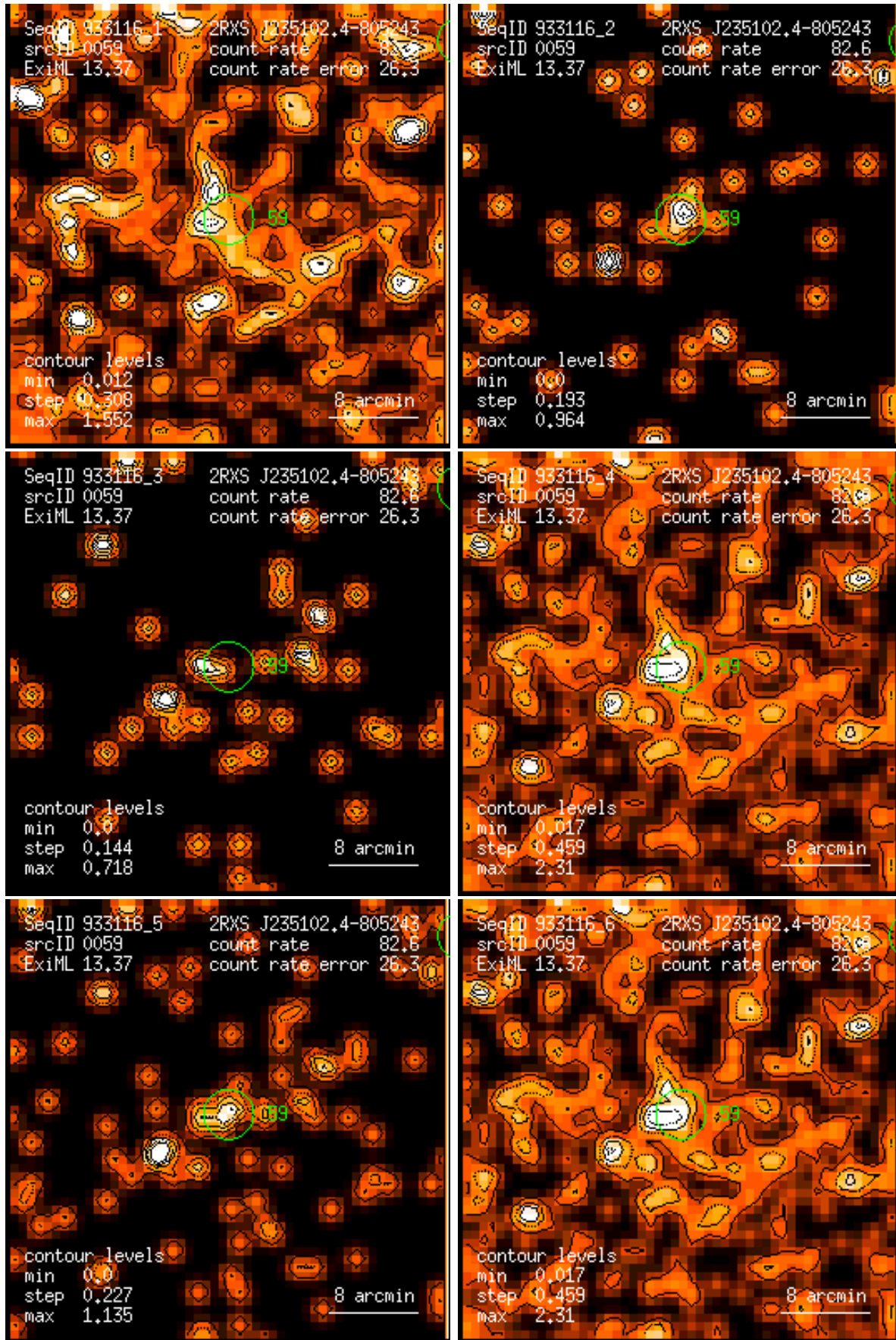
Figure 59: RASS 933116: detection 0059: band rate images, Gaussian filter: (1) PSPC channels 11 – 41, (2) 52 – 90, (3) 91 – 201, (4) 11 – 235, (5) 52 – 201, (6) 11 – 201. Broad band rates in counts/ks. Band rate contour levels in counts/ks/arcmin 2 .
