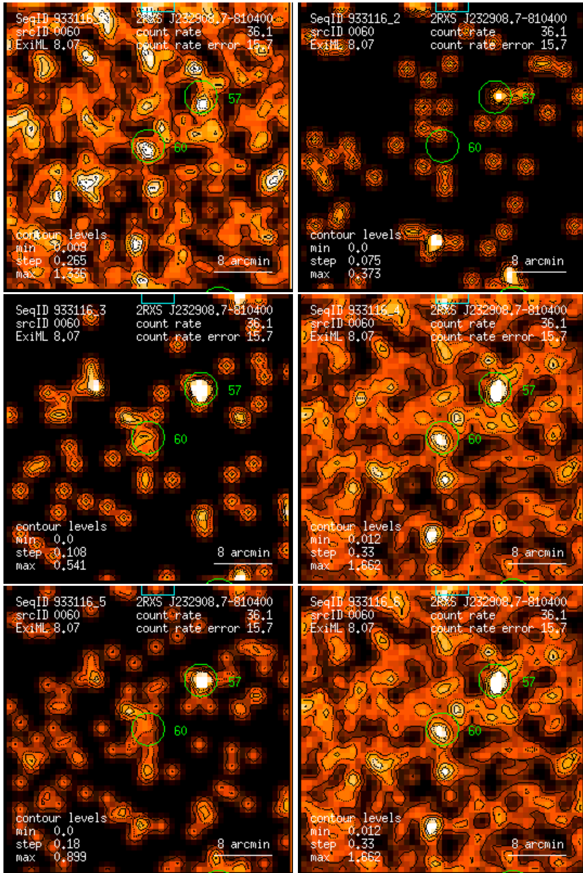
Figure 60: RASS 933116: detection 0060: band rate images, Gaussian filter: (1) PSPC channels 11 – 41, (2) 52 – 90, (3) 91 – 201, (4) 11 – 235, (5) 52 – 201, (6) 11 – 201. Broad band rates in counts/ks. Band rate contour levels in counts/ks/arcmin 2 .
