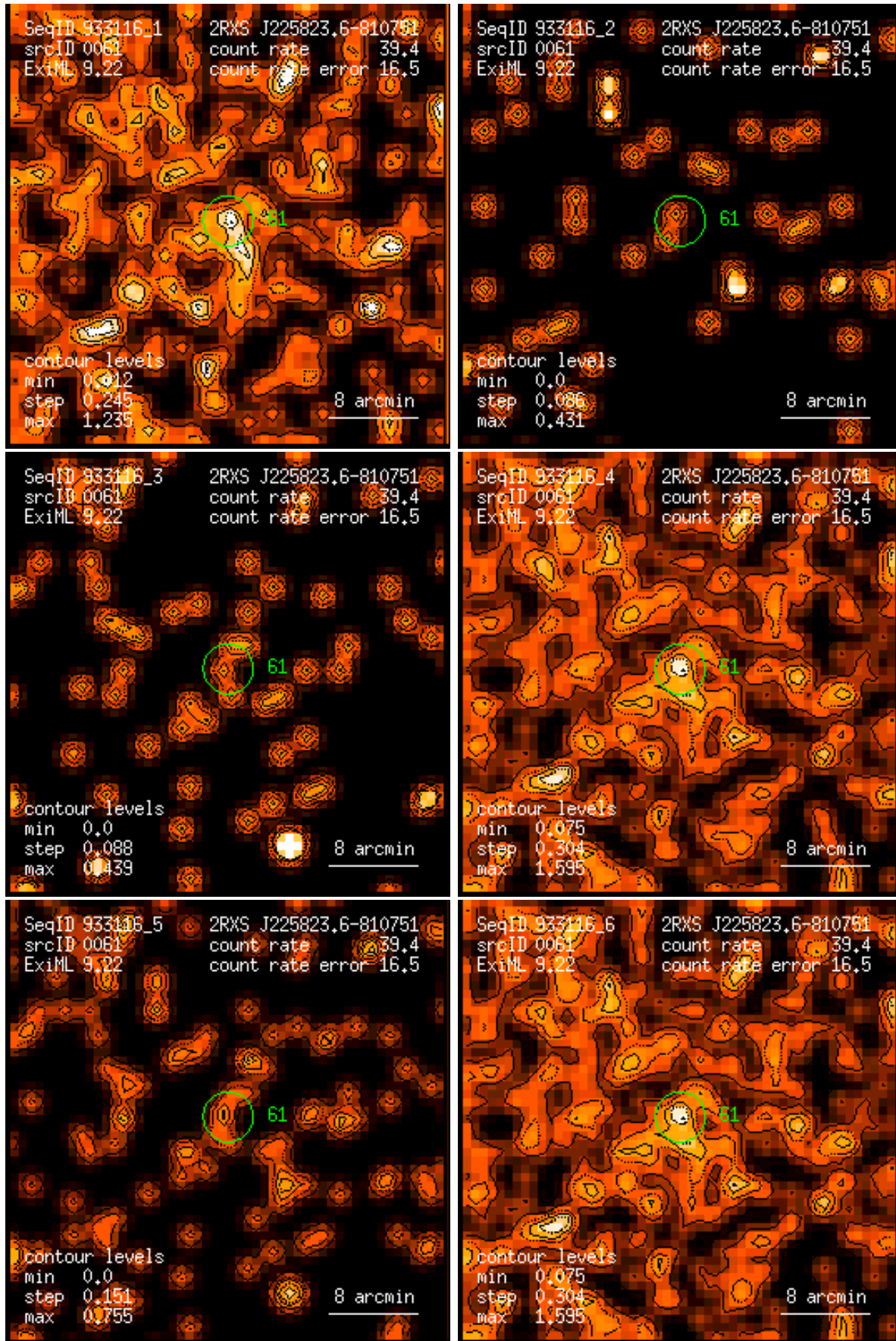
Figure 61: RASS 933116: detection 0061: band rate images, Gaussian filter: (1) PSPC channels 11 – 41, (2) 52 – 90, (3) 91 – 201, (4) 11 – 235, (5) 52 – 201, (6) 11 – 201. Broad band rates in counts/ks. Band rate contour levels in counts/ks/arcmin 2 .
