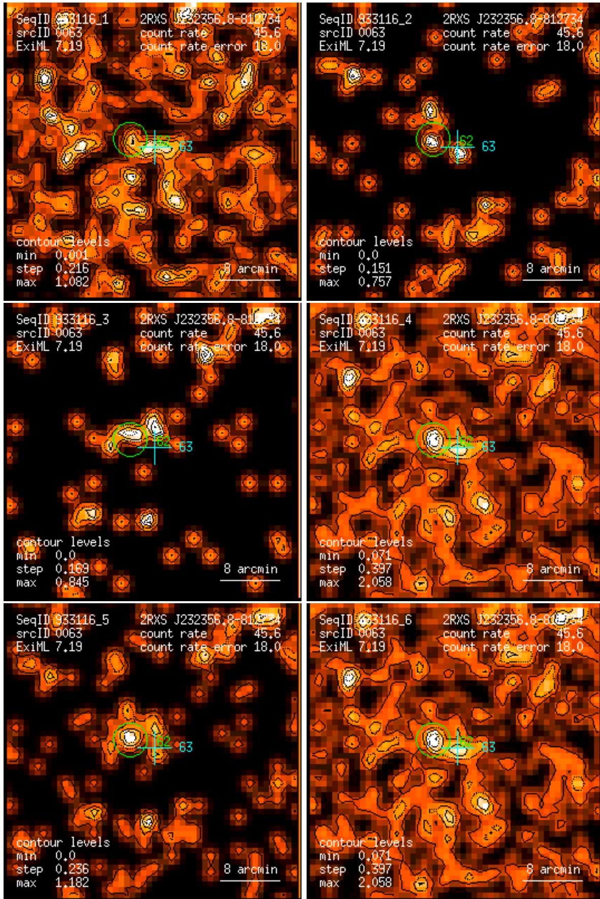
Figure 63: RASS 933116: detection 0063: band rate images, Gaussian filter: (1) PSPC channels 11 – 41, (2) 52 – 90, (3) 91 – 201, (4) 11 – 235, (5) 52 – 201, (6) 11 – 201. Broad band rates in counts/ks. Band rate contour levels in counts/ks/arcmin 2 .
