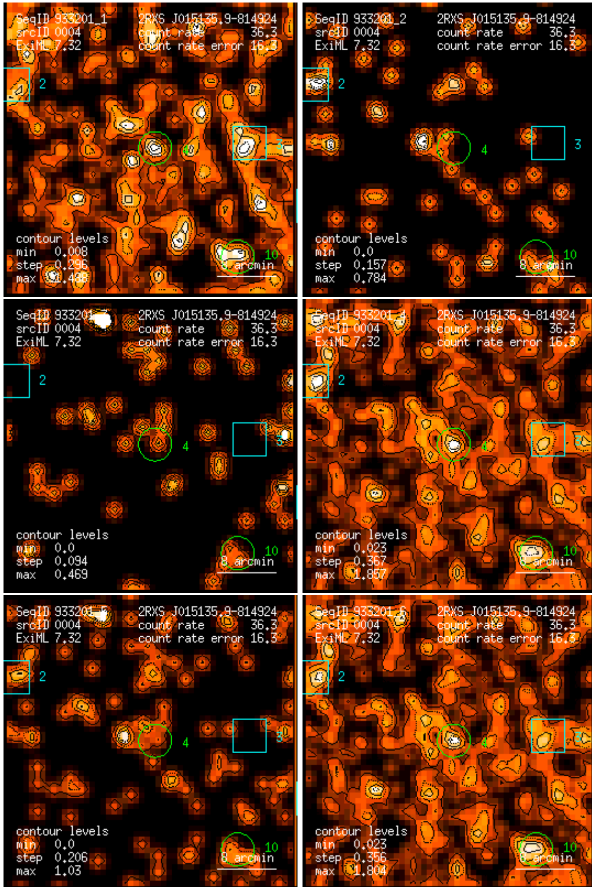
Figure 4: RASS 933201: detection 0004: band rate images, Gaussian filter: (1) PSPC channels 11 – 41, (2) 52 – 90, (3) 91 – 201, (4) 11 – 235, (5) 52 – 201, (6) 11 – 201. Broad band rates in counts/ks. Band rate contour levels in counts/ks/arcmin 2 .
