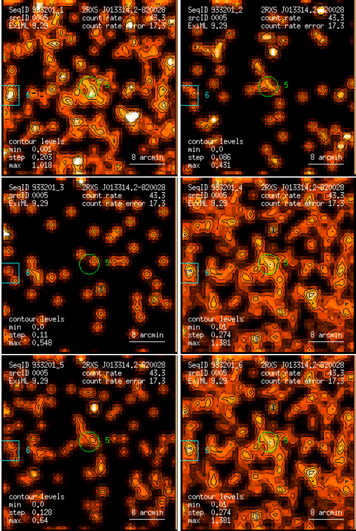
Figure 5: RASS 933201: detection 0005: band rate images, Gaussian filter: (1) PSPC channels 11 – 41, (2) 52 – 90, (3) 91 – 201, (4) 11 – 235, (5) 52 – 201, (6) 11 – 201. Broad band rates in counts/ks. Band rate contour levels in counts/ks/arcmin 2 .
