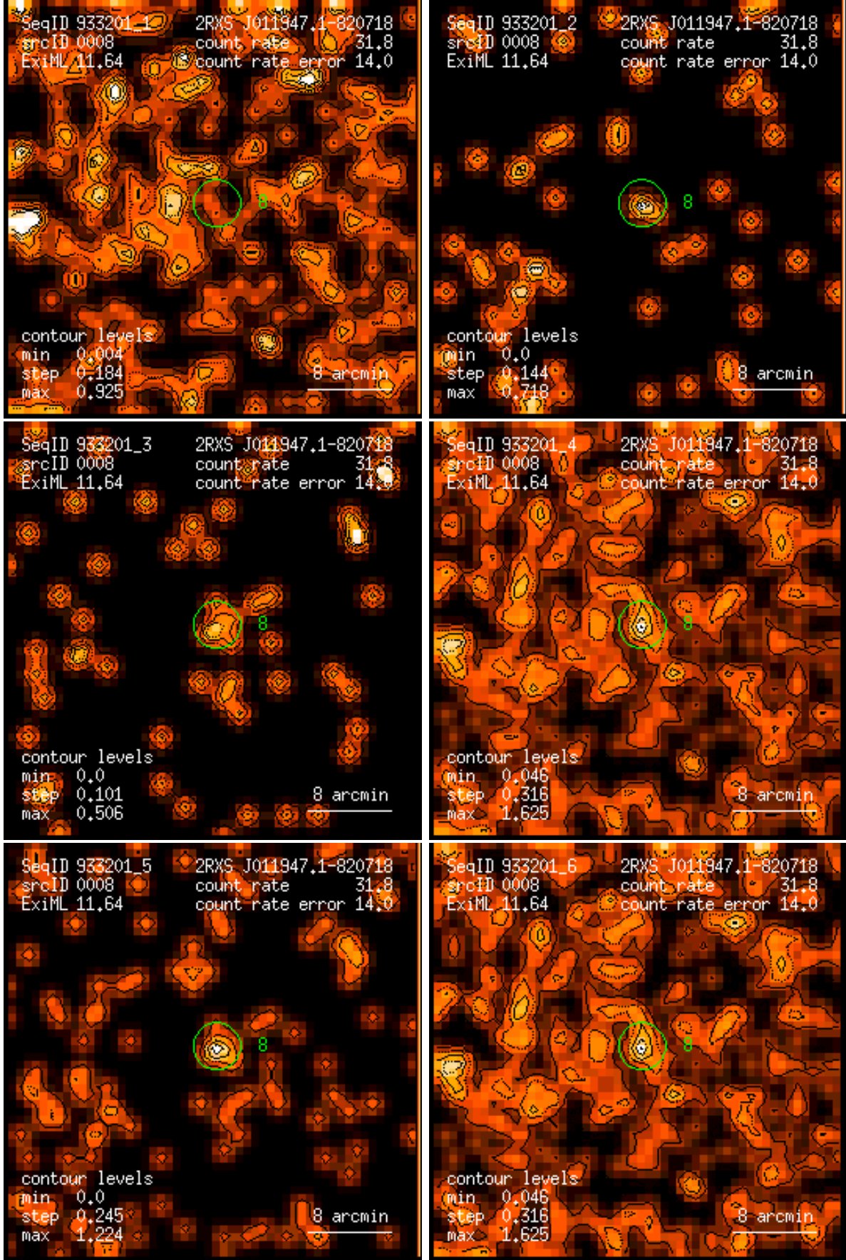
Figure 8: RASS 933201: detection 0008: band rate images, Gaussian filter: (1) PSPC channels 11 – 41, (2) 52 – 90, (3) 91 – 201, (4) 11 – 235, (5) 52 – 201, (6) 11 – 201. Broad band rates in counts/ks. Band rate contour levels in counts/ks/arcmin 2 .
