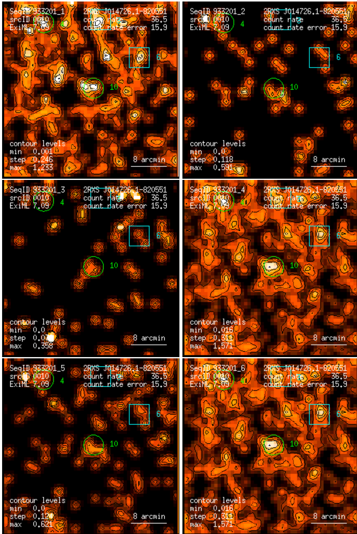
Figure 10: RASS 933201: detection 0010: band rate images, Gaussian filter: (1) PSPC channels 11 – 41, (2) 52 – 90, (3) 91 – 201, (4) 11 – 235, (5) 52 – 201, (6) 11 – 201. Broad band rates in counts/ks. Band rate contour levels in counts/ks/arcmin 2 .
