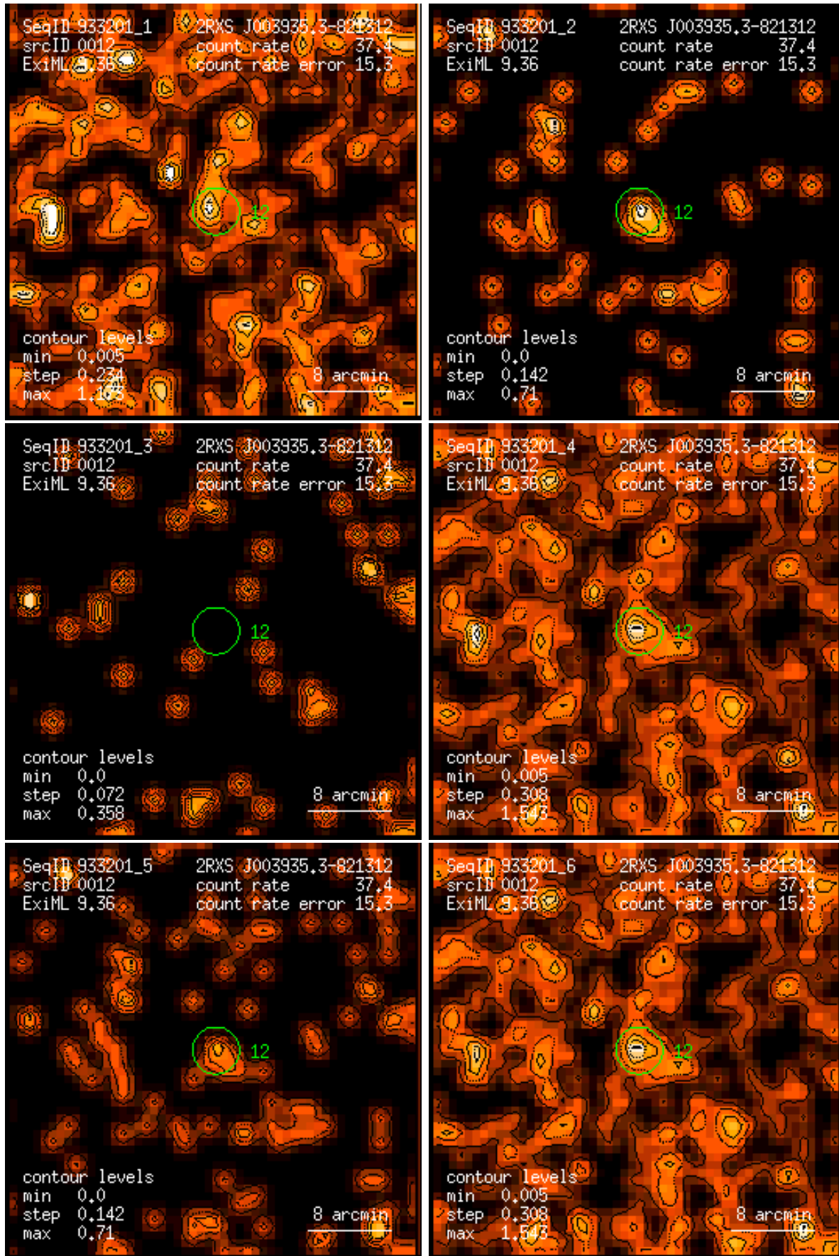
Figure 12: RASS 933201: detection 0012: band rate images, Gaussian filter: (1) PSPC channels 11 – 41, (2) 52 – 90, (3) 91 – 201, (4) 11 – 235, (5) 52 – 201, (6) 11 – 201. Broad band rates in counts/ks. Band rate contour levels in counts/ks/arcmin 2 .
