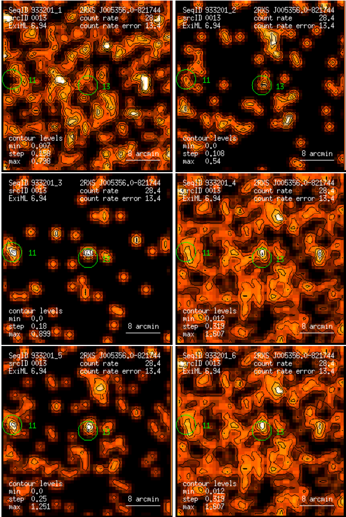
Figure 13: RASS 933201: detection 0013: band rate images, Gaussian filter: (1) PSPC channels 11 – 41, (2) 52 – 90, (3) 91 – 201, (4) 11 – 235, (5) 52 – 201, (6) 11 – 201. Broad band rates in counts/ks. Band rate contour levels in counts/ks/arcmin 2 .
