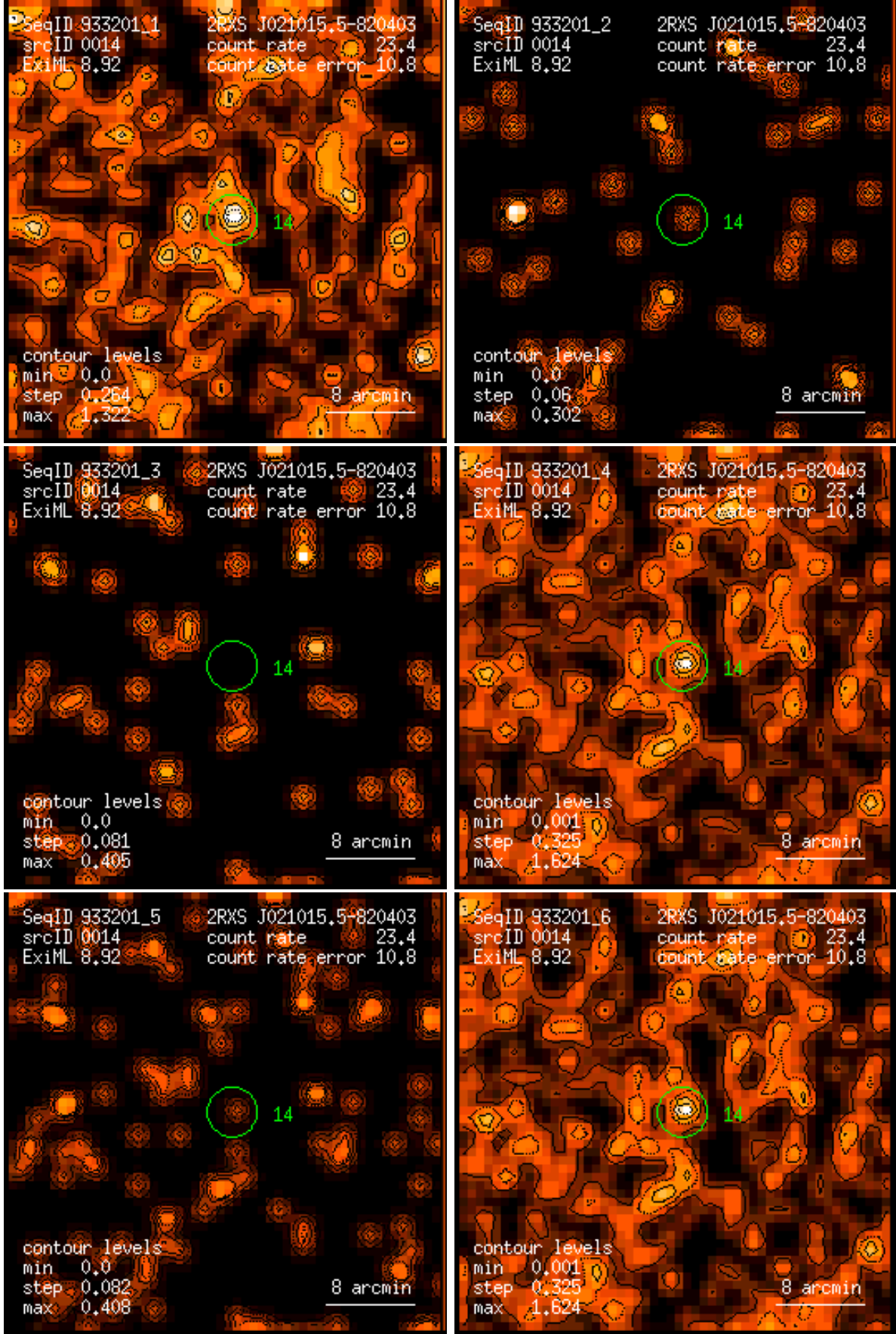
Figure 14: RASS 933201: detection 0014: band rate images, Gaussian filter: (1) PSPC channels 11 – 41, (2) 52 – 90, (3) 91 – 201, (4) 11 – 235, (5) 52 – 201, (6) 11 – 201. Broad band rates in counts/ks. Band rate contour levels in counts/ks/arcmin 2 .
