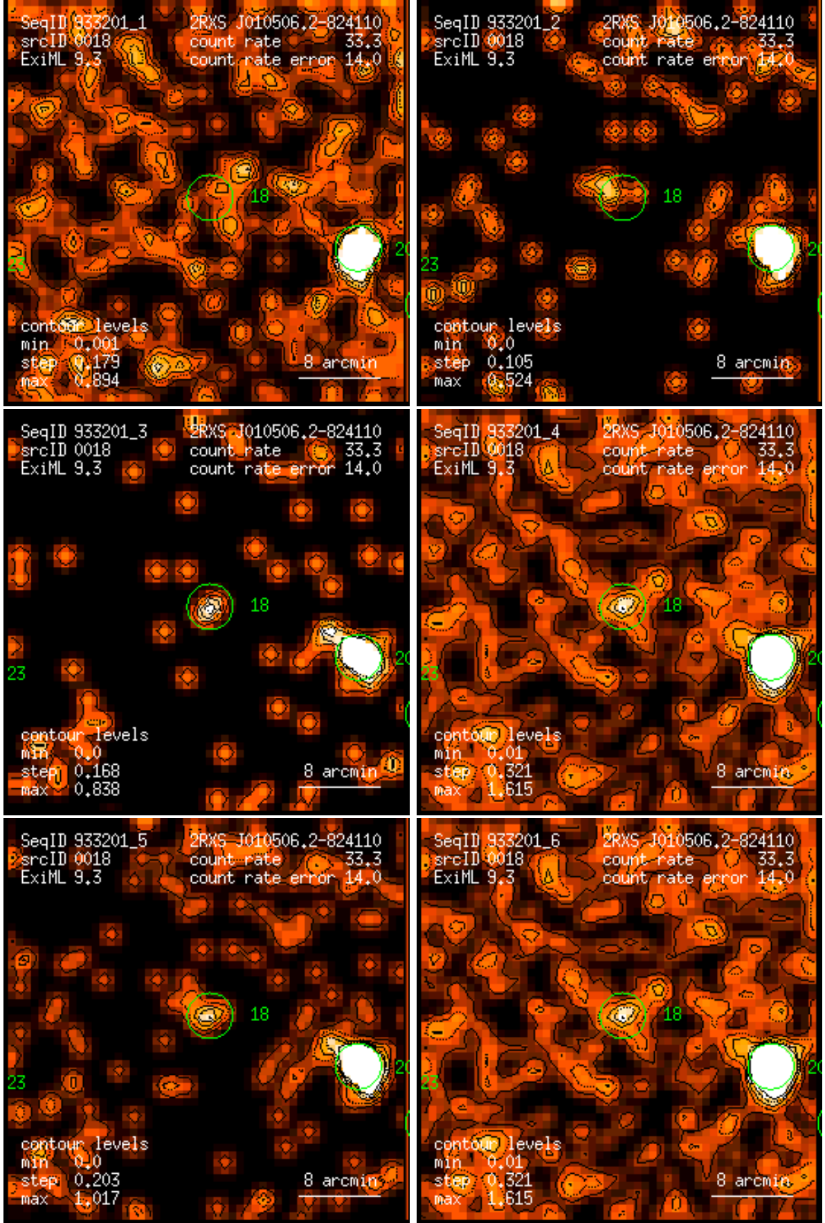
Figure 18: RASS 933201: detection 0018: band rate images, Gaussian filter: (1) PSPC channels 11 – 41, (2) 52 – 90, (3) 91 – 201, (4) 11 – 235, (5) 52 – 201, (6) 11 – 201. Broad band rates in counts/ks. Band rate contour levels in counts/ks/arcmin 2 .
