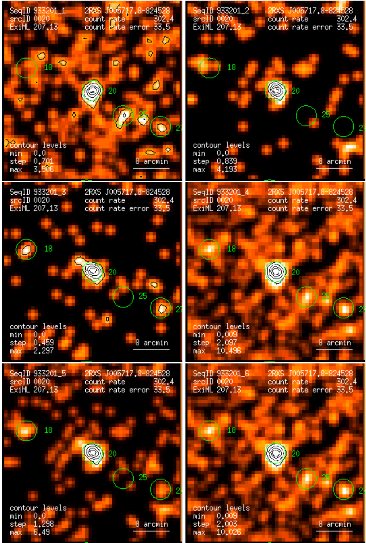
Figure 20: RASS 933201: detection 0020: band rate images, Gaussian filter: (1) PSPC channels 11 – 41, (2) 52 – 90, (3) 91 – 201, (4) 11 – 235, (5) 52 – 201, (6) 11 – 201. Broad band rates in counts/ks. Band rate contour levels in counts/ks/arcmin 2 .
