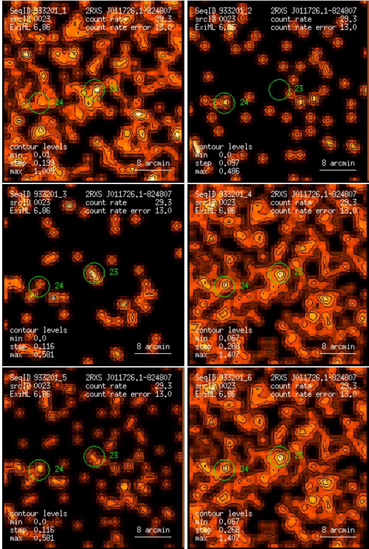
Figure 23: RASS 933201: detection 0023: band rate images, Gaussian filter: (1) PSPC channels 11 – 41, (2) 52 – 90, (3) 91 – 201, (4) 11 – 235, (5) 52 – 201, (6) 11 – 201. Broad band rates in counts/ks. Band rate contour levels in counts/ks/arcmin 2 .
