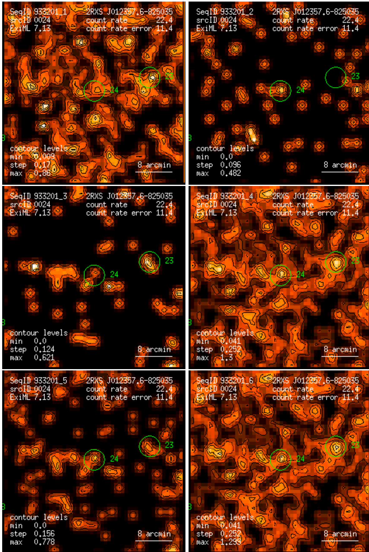
Figure 24: RASS 933201: detection 0024: band rate images, Gaussian filter: (1) PSPC channels 11 – 41, (2) 52 – 90, (3) 91 – 201, (4) 11 – 235, (5) 52 – 201, (6) 11 – 201. Broad band rates in counts/ks. Band rate contour levels in counts/ks/arcmin 2 .
