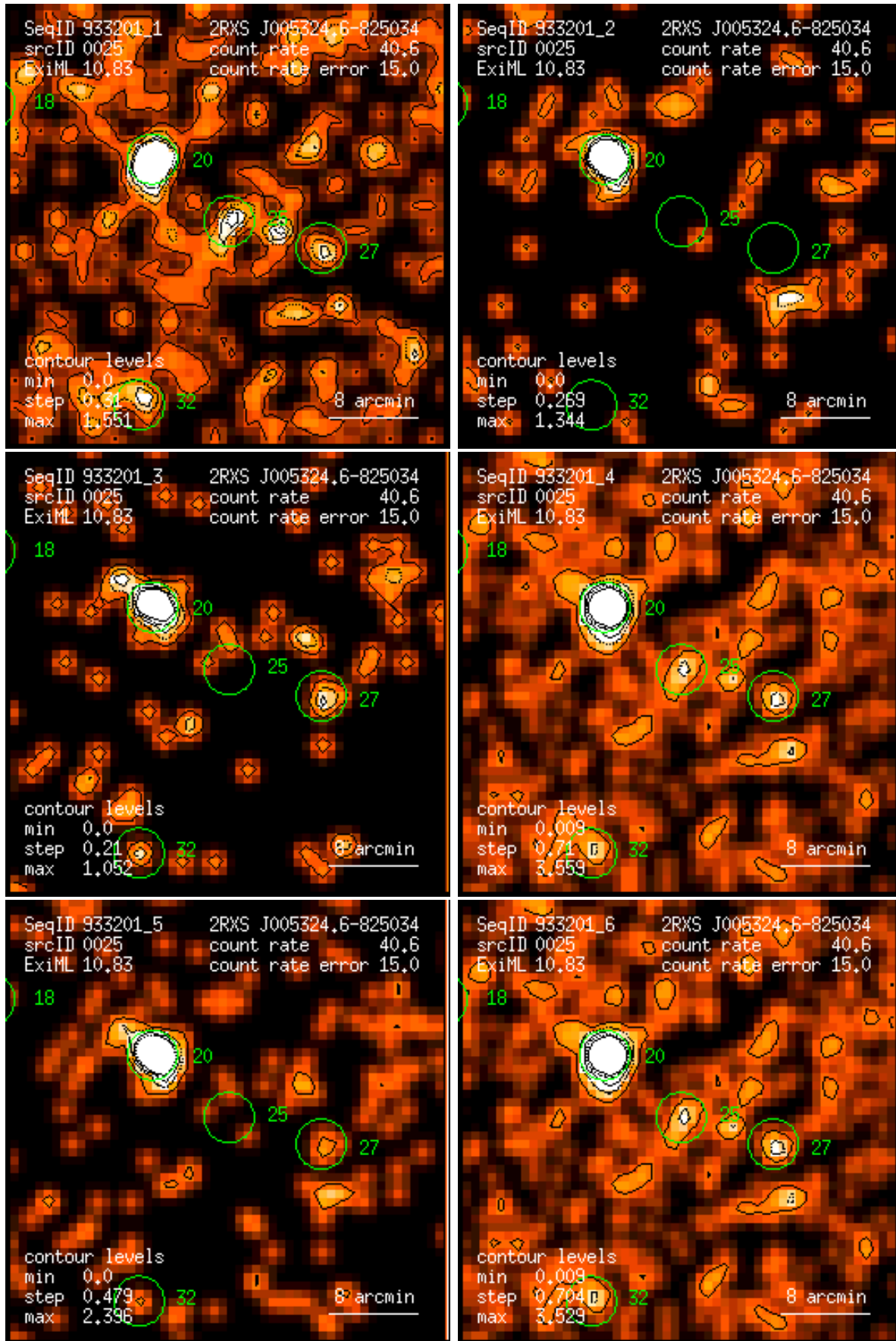
Figure 25: RASS 933201: detection 0025: band rate images, Gaussian filter: (1) PSPC channels 11 – 41, (2) 52 – 90, (3) 91 – 201, (4) 11 – 235, (5) 52 – 201, (6) 11 – 201. Broad band rates in counts/ks. Band rate contour levels in counts/ks/arcmin 2 .
