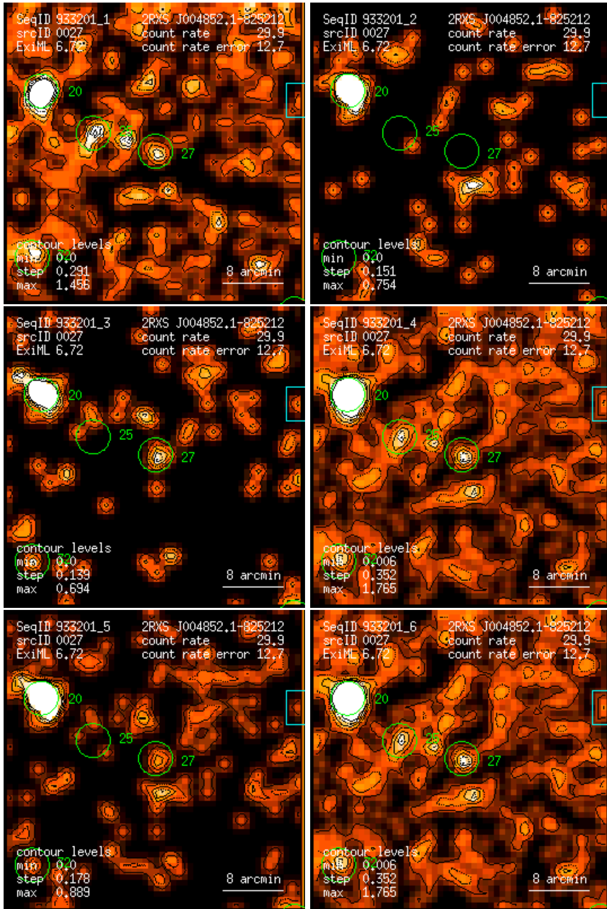
Figure 27: RASS 933201: detection 0027: band rate images, Gaussian filter: (1) PSPC channels 11 – 41, (2) 52 – 90, (3) 91 – 201, (4) 11 – 235, (5) 52 – 201, (6) 11 – 201. Broad band rates in counts/ks. Band rate contour levels in counts/ks/arcmin 2 .
