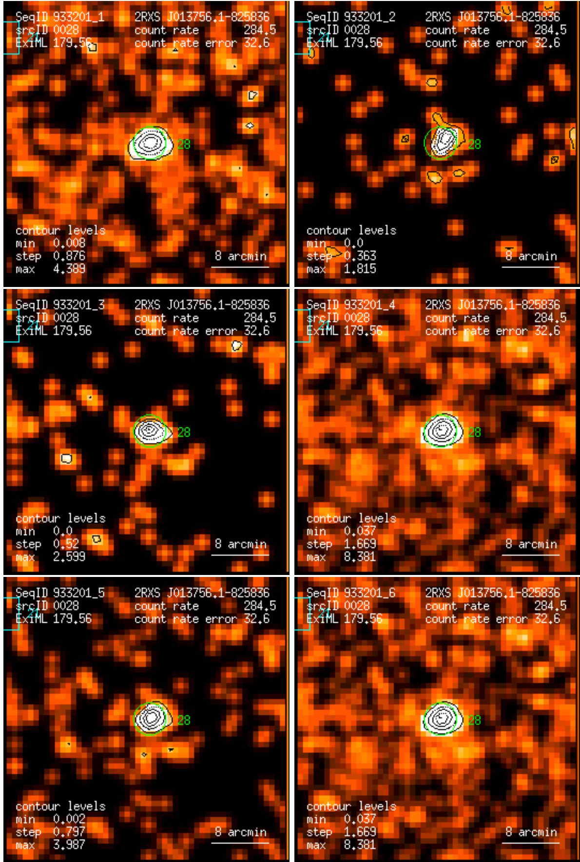
Figure 28: RASS 933201: detection 0028: band rate images, Gaussian filter: (1) PSPC channels 11 – 41, (2) 52 – 90, (3) 91 – 201, (4) 11 – 235, (5) 52 – 201, (6) 11 – 201. Broad band rates in counts/ks. Band rate contour levels in counts/ks/arcmin 2 .
