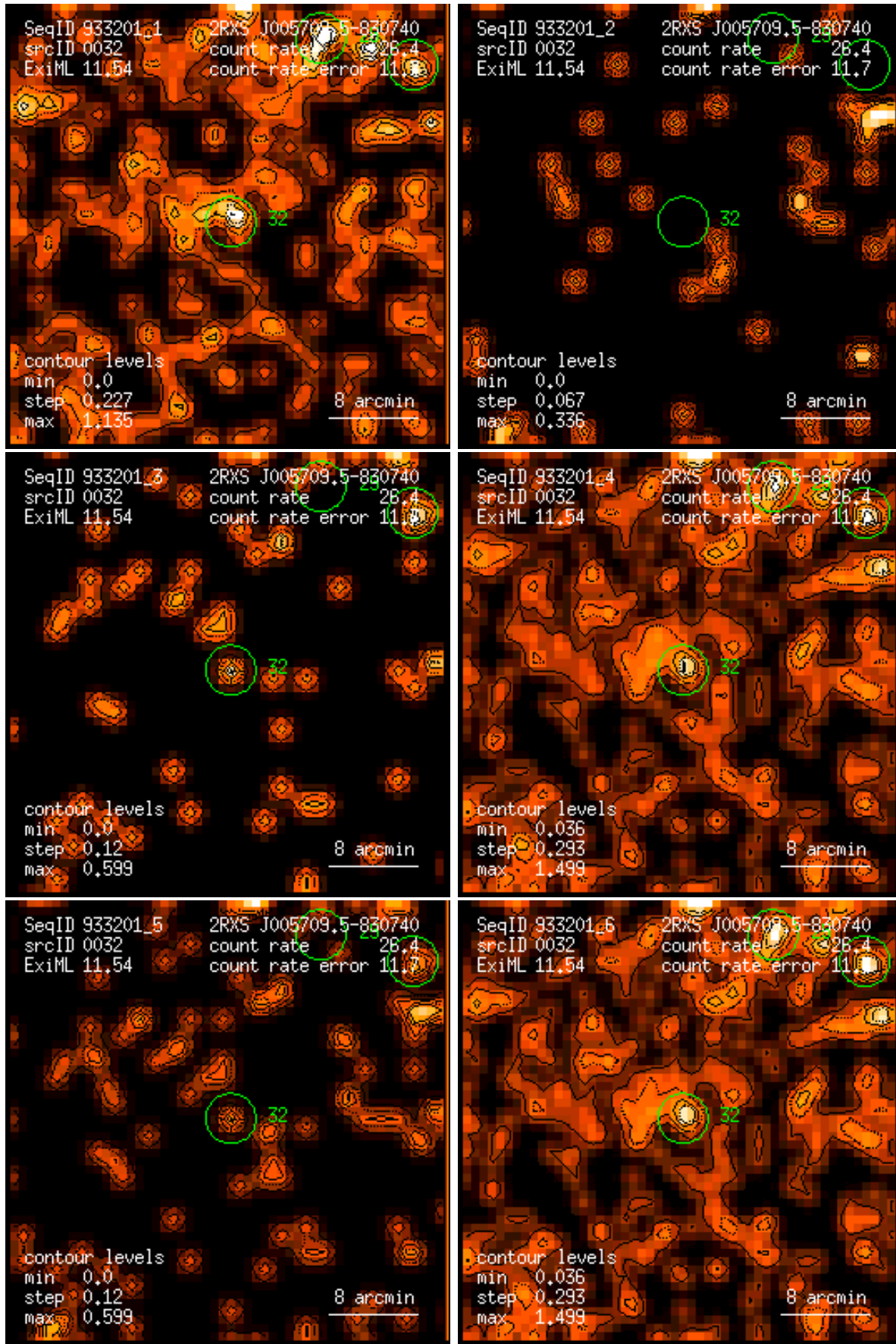
Figure 32: RASS 933201: detection 0032: band rate images, Gaussian filter: (1) PSPC channels 11 – 41, (2) 52 – 90, (3) 91 – 201, (4) 11 – 235, (5) 52 – 201, (6) 11 – 201. Broad band rates in counts/ks. Band rate contour levels in counts/ks/arcmin 2 .
