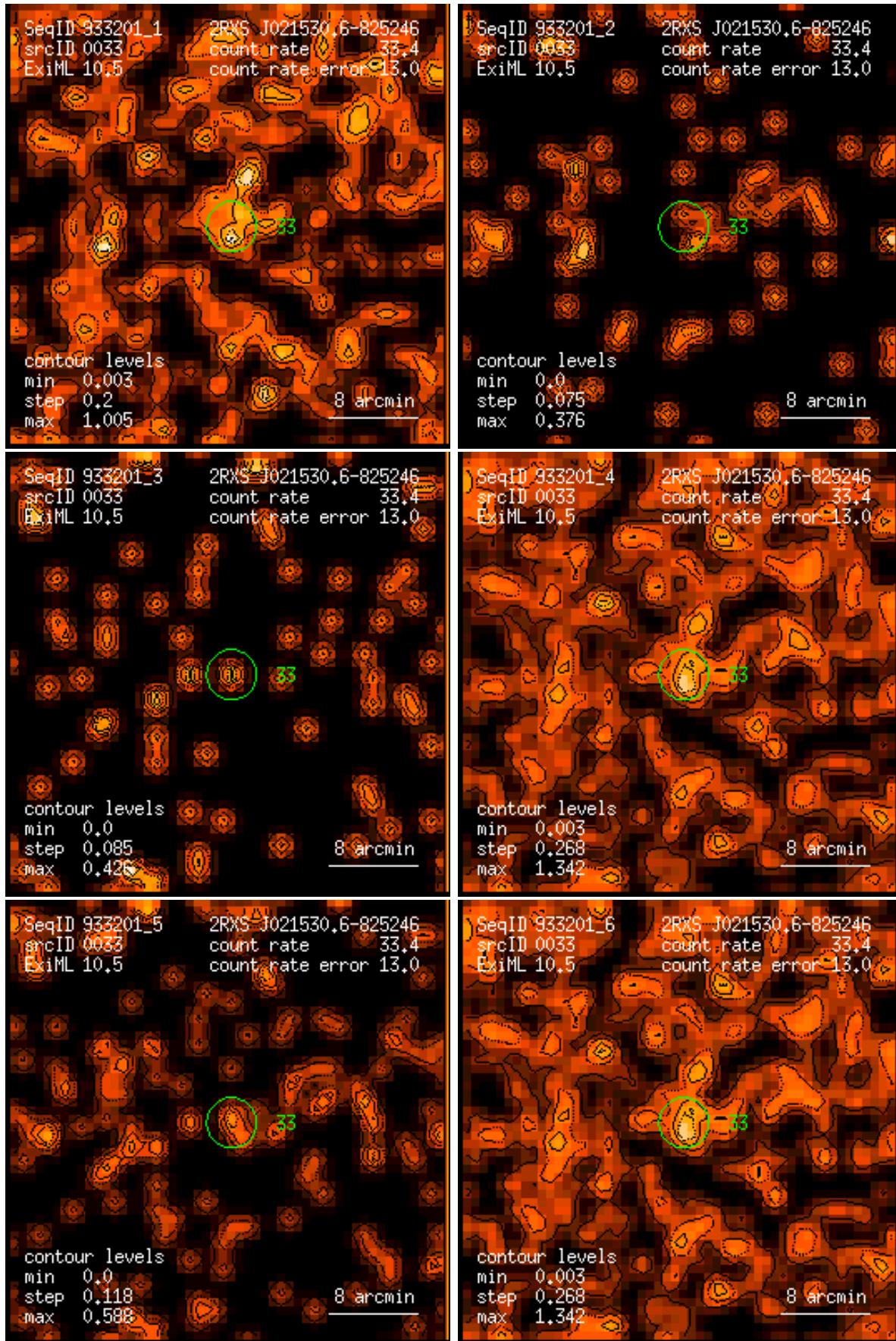
Figure 33: RASS 933201: detection 0033: band rate images, Gaussian filter: (1) PSPC channels 11 – 41, (2) 52 – 90, (3) 91 – 201, (4) 11 – 235, (5) 52 – 201, (6) 11 – 201. Broad band rates in counts/ks. Band rate contour levels in counts/ks/arcmin 2 .
