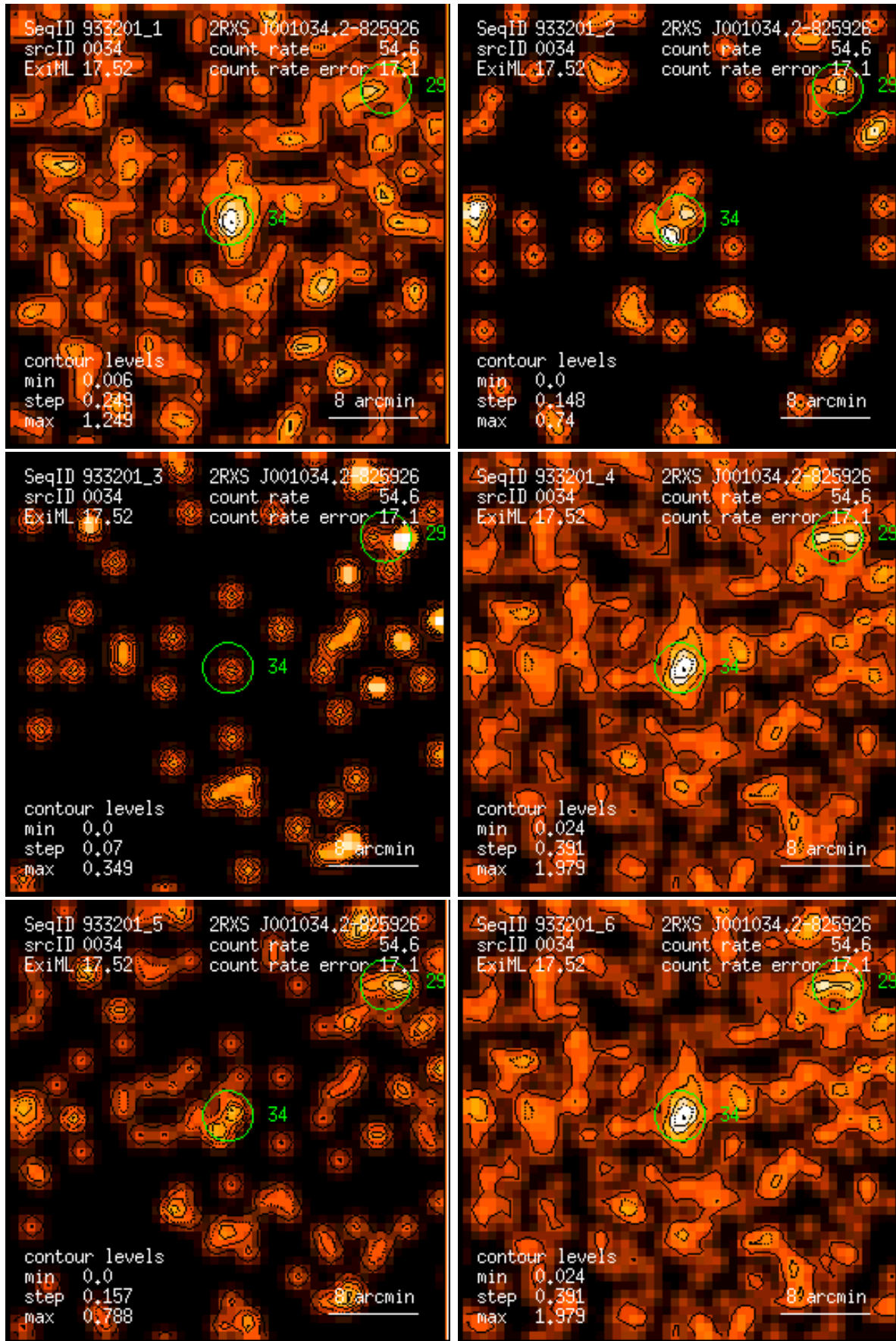
Figure 34: RASS 933201: detection 0034: band rate images, Gaussian filter: (1) PSPC channels 11 – 41, (2) 52 – 90, (3) 91 – 201, (4) 11 – 235, (5) 52 – 201, (6) 11 – 201. Broad band rates in counts/ks. Band rate contour levels in counts/ks/arcmin 2 .
