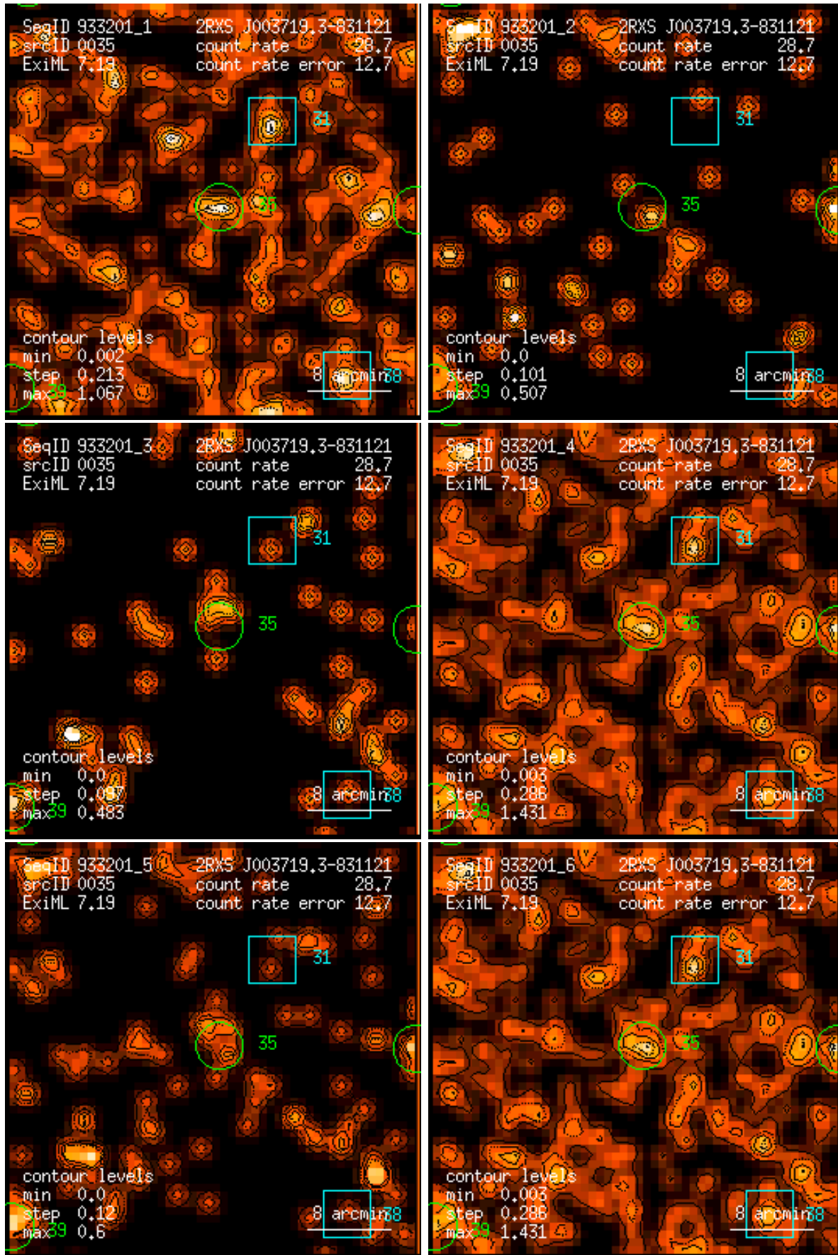
Figure 35: RASS 933201: detection 0035: band rate images, Gaussian filter: (1) PSPC channels 11 – 41, (2) 52 – 90, (3) 91 – 201, (4) 11 – 235, (5) 52 – 201, (6) 11 – 201. Broad band rates in counts/ks. Band rate contour levels in counts/ks/arcmin 2 .
