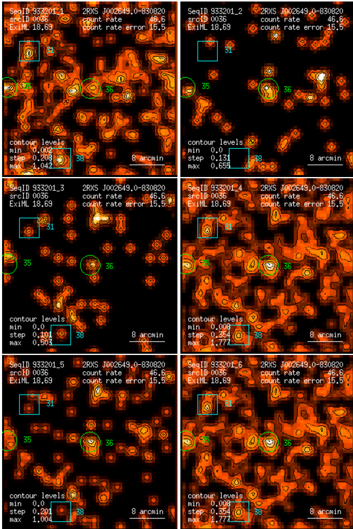
Figure 36: RASS 933201: detection 0036: band rate images, Gaussian filter: (1) PSPC channels 11 – 41, (2) 52 – 90, (3) 91 – 201, (4) 11 – 235, (5) 52 – 201, (6) 11 – 201. Broad band rates in counts/ks. Band rate contour levels in counts/ks/arcmin 2 .
