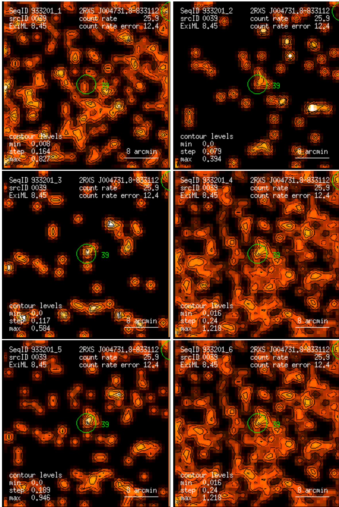
Figure 39: RASS 933201: detection 0039: band rate images, Gaussian filter: (1) PSPC channels 11 – 41, (2) 52 – 90, (3) 91 – 201, (4) 11 – 235, (5) 52 – 201, (6) 11 – 201. Broad band rates in counts/ks. Band rate contour levels in counts/ks/arcmin 2 .
