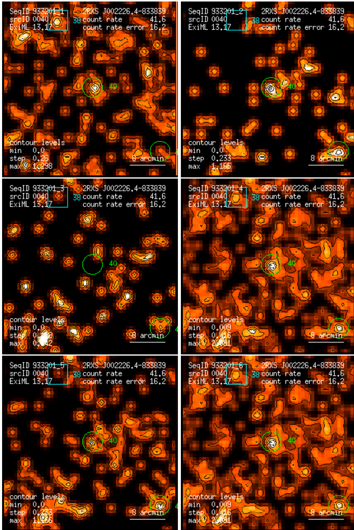
Figure 40: RASS 933201: detection 0040: band rate images, Gaussian filter: (1) PSPC channels 11 – 41, (2) 52 – 90, (3) 91 – 201, (4) 11 – 235, (5) 52 – 201, (6) 11 – 201. Broad band rates in counts/ks. Band rate contour levels in counts/ks/arcmin 2 .
