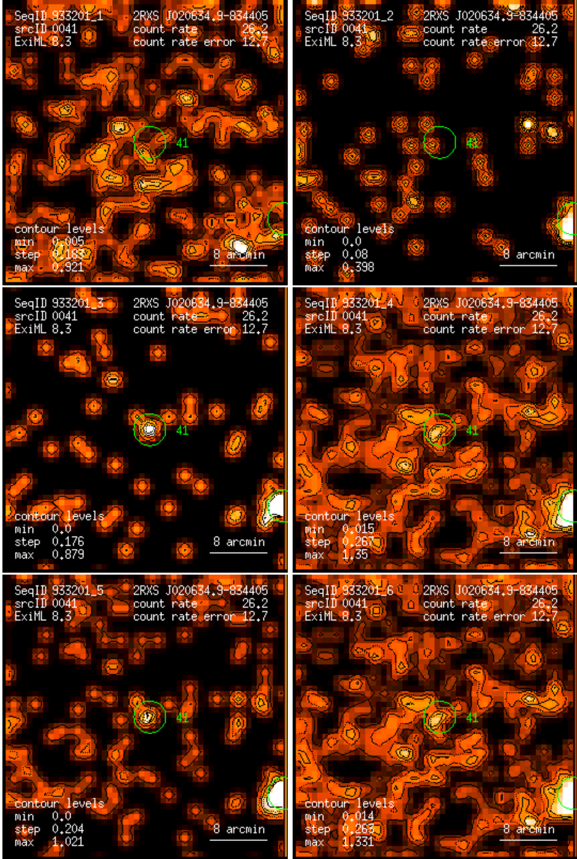
Figure 41: RASS 933201: detection 0041: band rate images, Gaussian filter: (1) PSPC channels 11 – 41, (2) 52 – 90, (3) 91 – 201, (4) 11 – 235, (5) 52 – 201, (6) 11 – 201. Broad band rates in counts/ks. Band rate contour levels in counts/ks/arcmin 2 .
