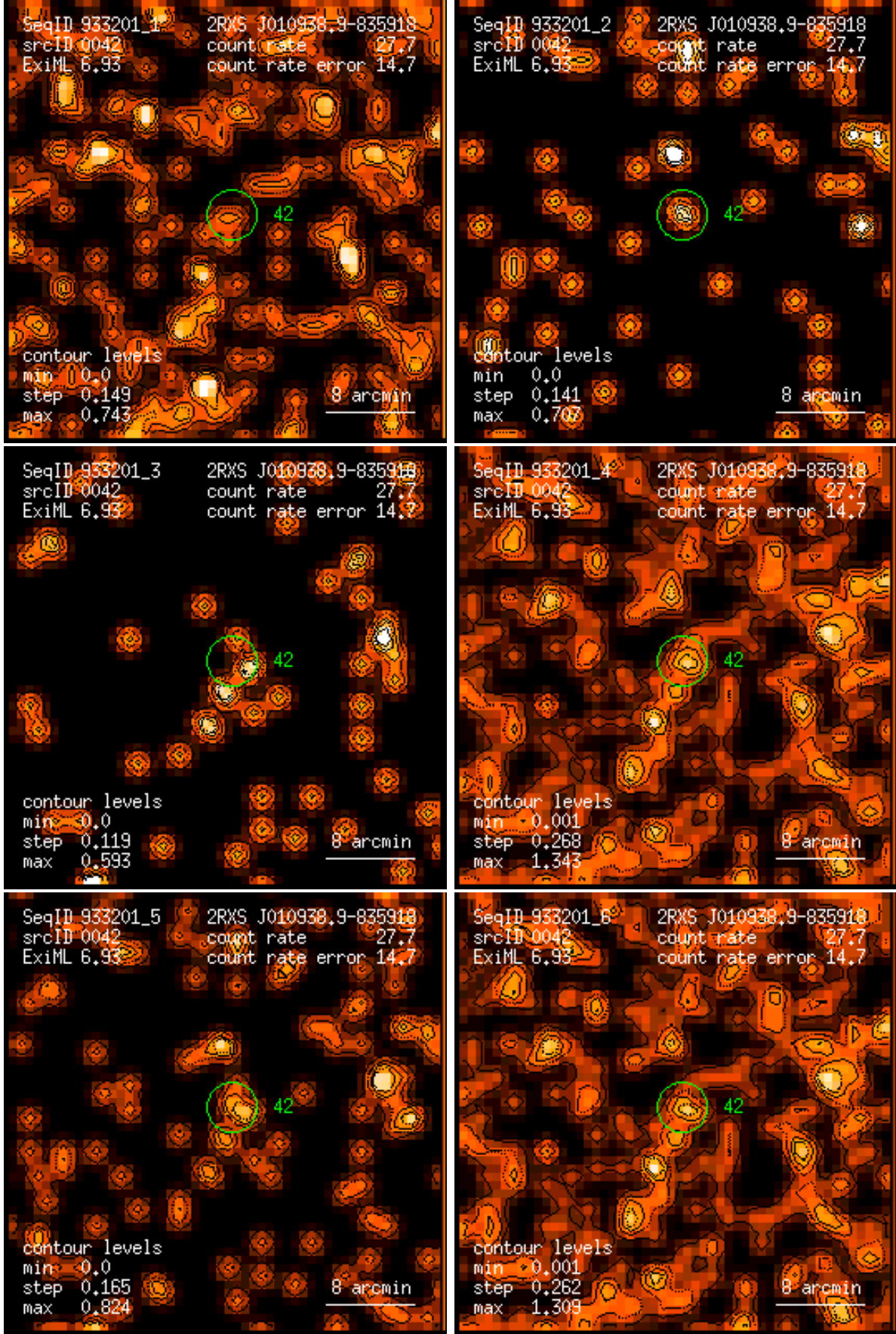
Figure 42: RASS 933201: detection 0042: band rate images, Gaussian filter: (1) PSPC channels 11 – 41, (2) 52 – 90, (3) 91 – 201, (4) 11 – 235, (5) 52 – 201, (6) 11 – 201. Broad band rates in counts/ks. Band rate contour levels in counts/ks/arcmin 2 .
