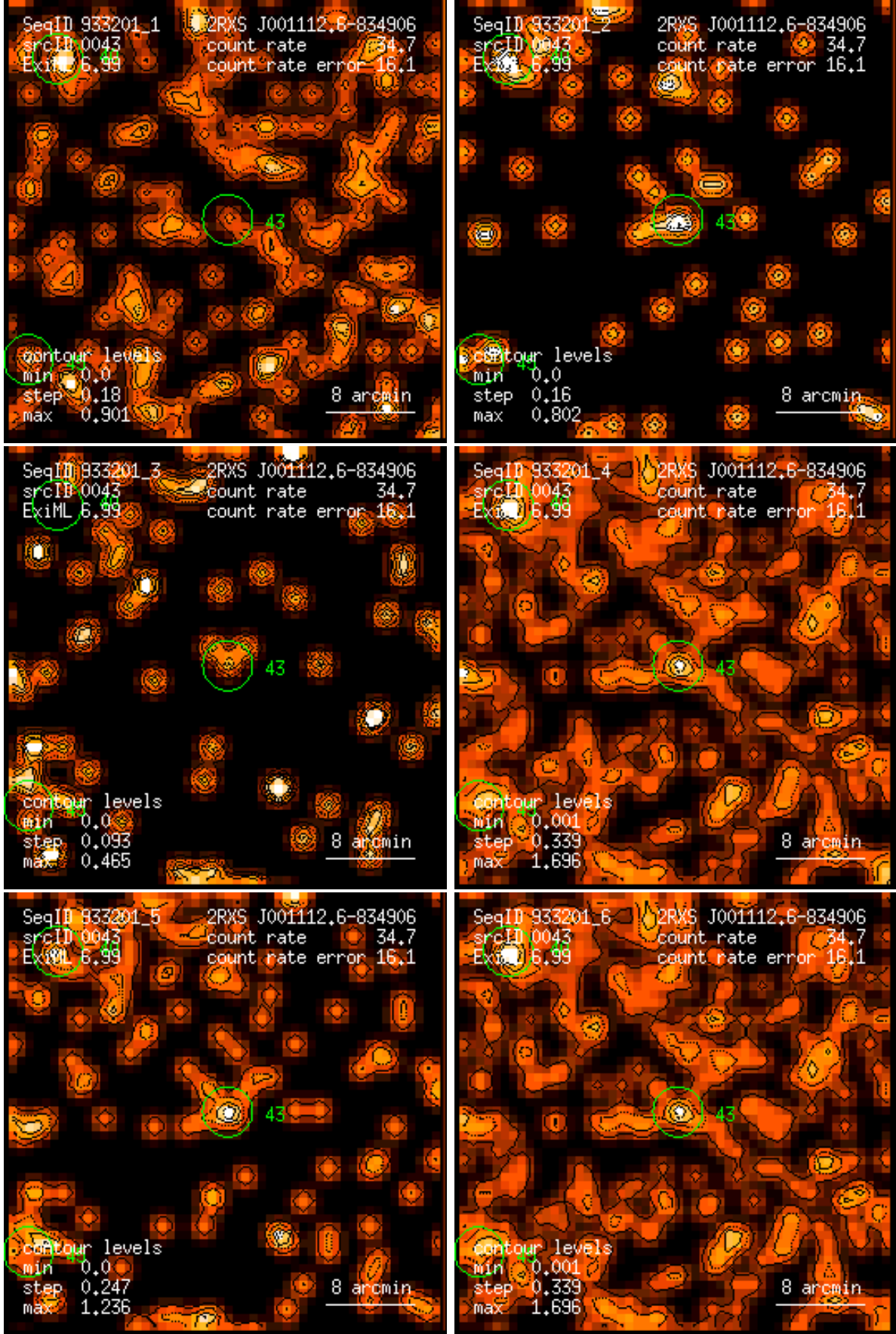
Figure 43: RASS 933201: detection 0043: band rate images, Gaussian filter: (1) PSPC channels 11 – 41, (2) 52 – 90, (3) 91 – 201, (4) 11 – 235, (5) 52 – 201, (6) 11 – 201. Broad band rates in counts/ks. Band rate contour levels in counts/ks/arcmin 2 .
