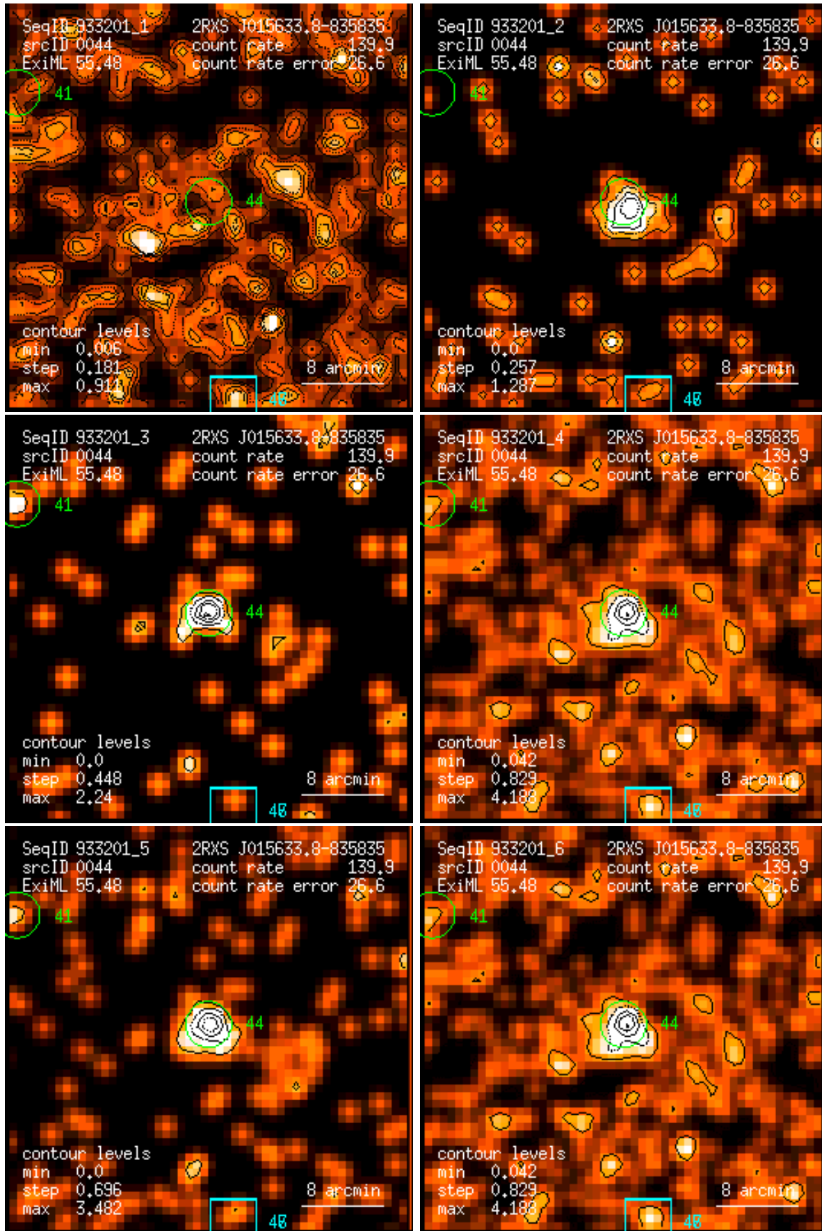
Figure 44: RASS 933201: detection 0044: band rate images, Gaussian filter: (1) PSPC channels 11 – 41, (2) 52 – 90, (3) 91 – 201, (4) 11 – 235, (5) 52 – 201, (6) 11 – 201. Broad band rates in counts/ks. Band rate contour levels in counts/ks/arcmin 2 .
