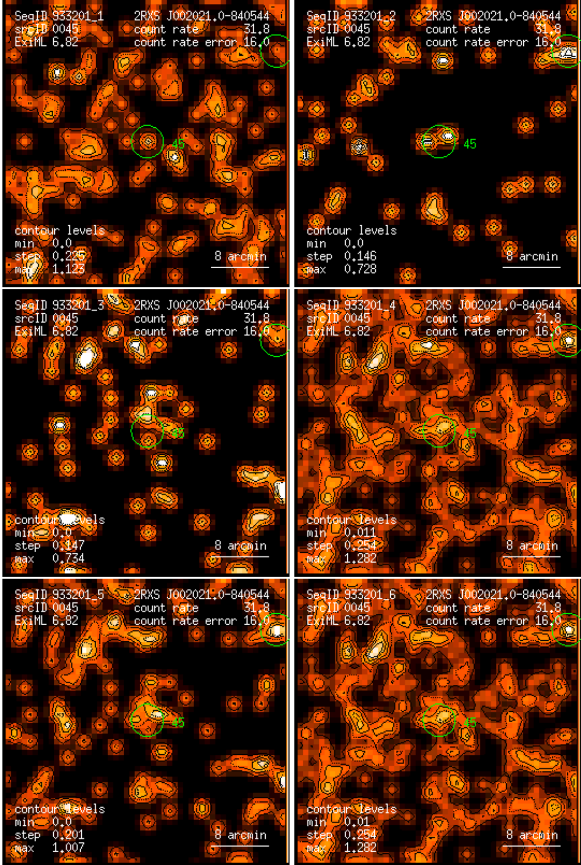
Figure 45: RASS 933201: detection 0045: band rate images, Gaussian filter: (1) PSPC channels 11 – 41, (2) 52 – 90, (3) 91 – 201, (4) 11 – 235, (5) 52 – 201, (6) 11 – 201. Broad band rates in counts/ks. Band rate contour levels in counts/ks/arcmin 2 .
