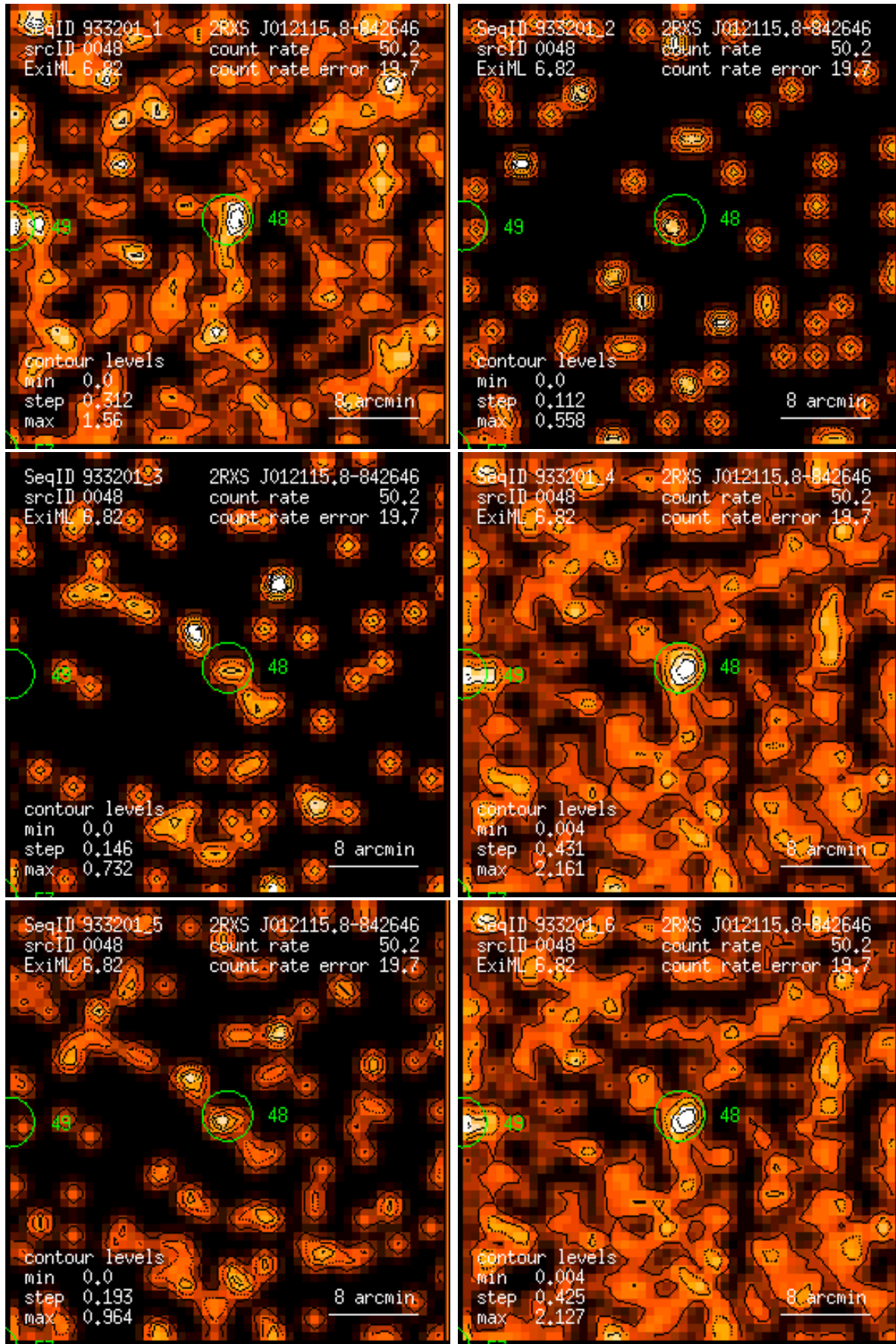
Figure 48: RASS 933201: detection 0048: band rate images, Gaussian filter: (1) PSPC channels 11 – 41, (2) 52 – 90, (3) 91 – 201, (4) 11 – 235, (5) 52 – 201, (6) 11 – 201. Broad band rates in counts/ks. Band rate contour levels in counts/ks/arcmin 2 .
