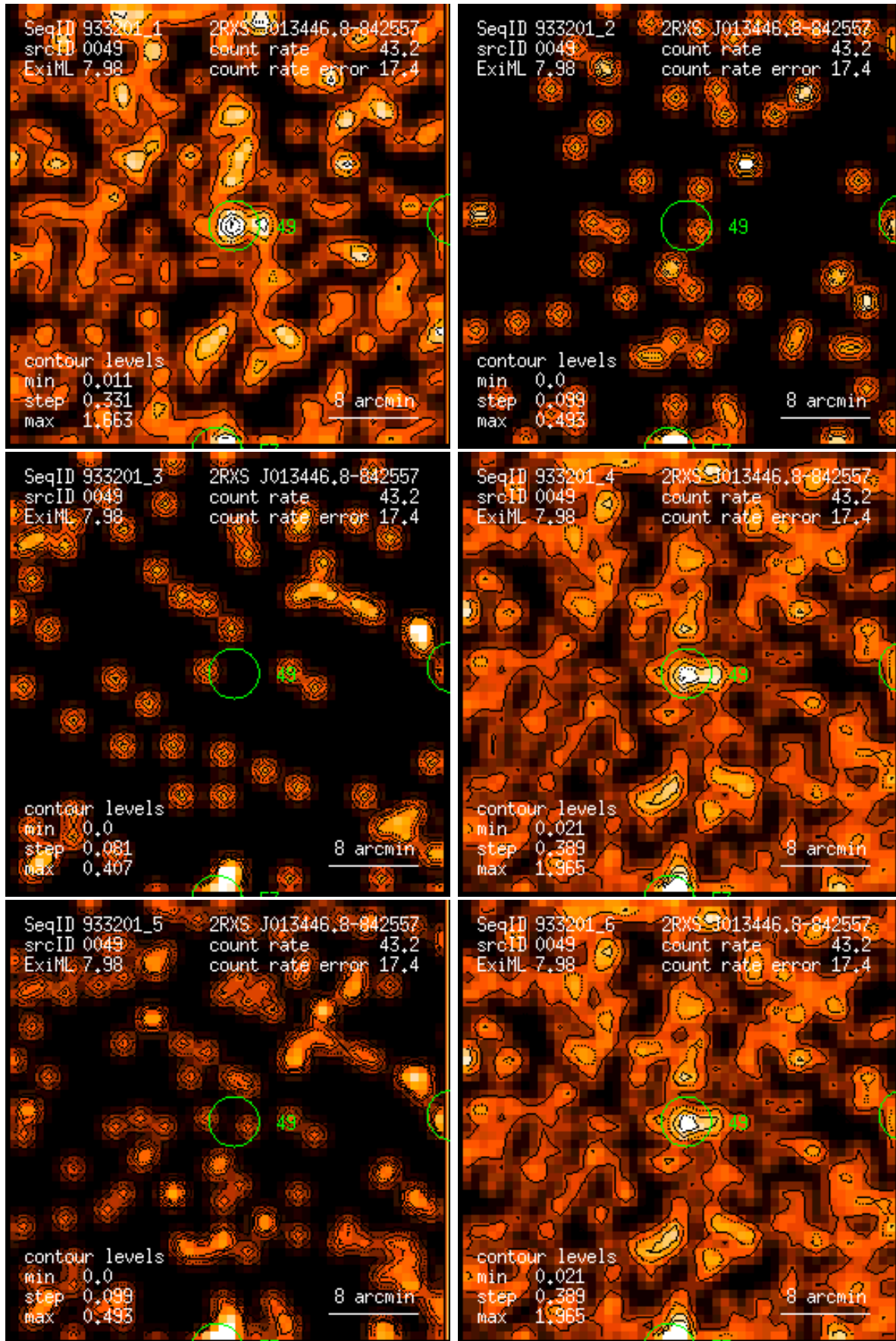
Figure 49: RASS 933201: detection 0049: band rate images, Gaussian filter: (1) PSPC channels 11 – 41, (2) 52 – 90, (3) 91 – 201, (4) 11 – 235, (5) 52 – 201, (6) 11 – 201. Broad band rates in counts/ks. Band rate contour levels in counts/ks/arcmin 2 .
