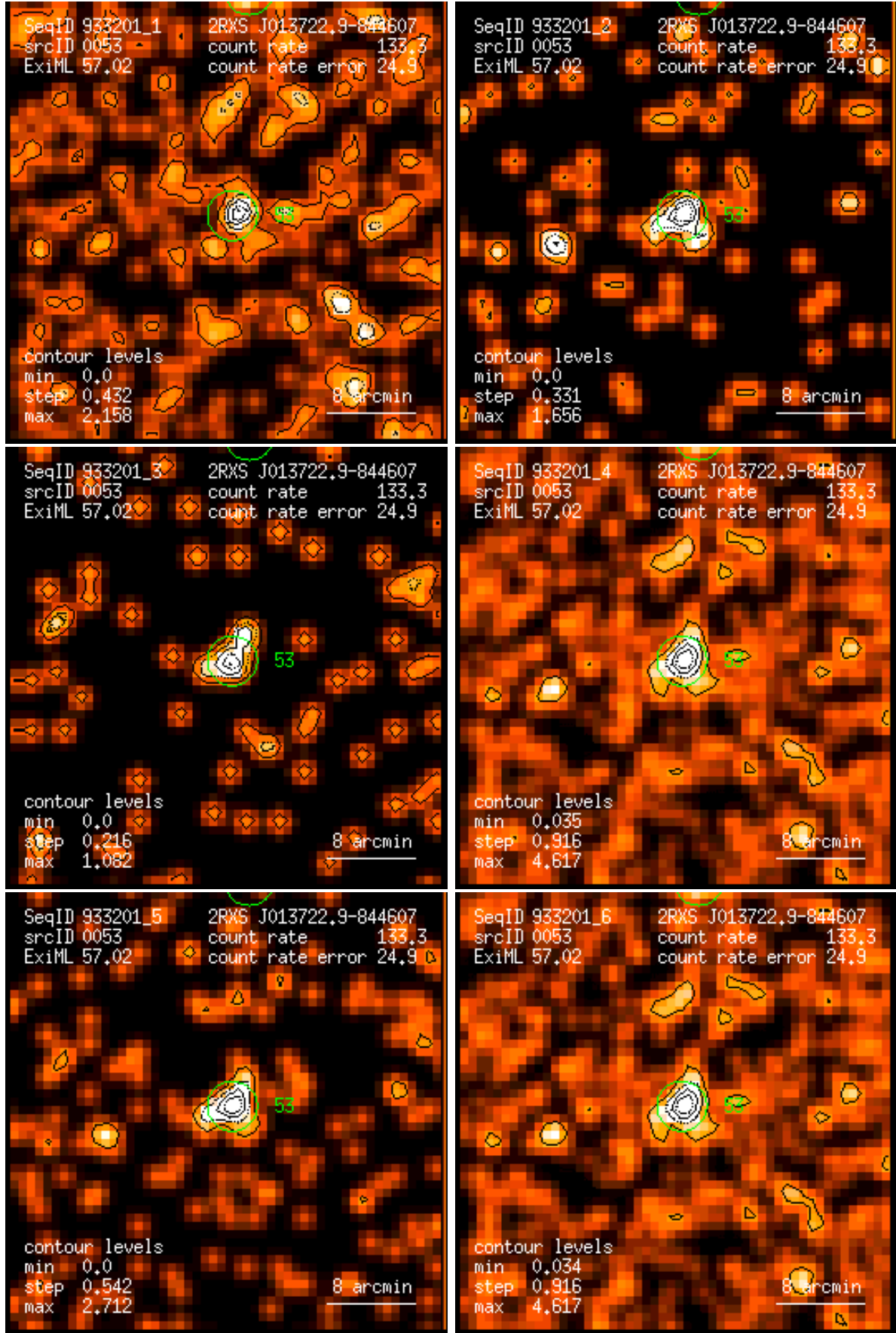
Figure 53: RASS 933201: detection 0053: band rate images, Gaussian filter: (1) PSPC channels 11 – 41, (2) 52 – 90, (3) 91 – 201, (4) 11 – 235, (5) 52 – 201, (6) 11 – 201. Broad band rates in counts/ks. Band rate contour levels in counts/ks/arcmin 2 .
