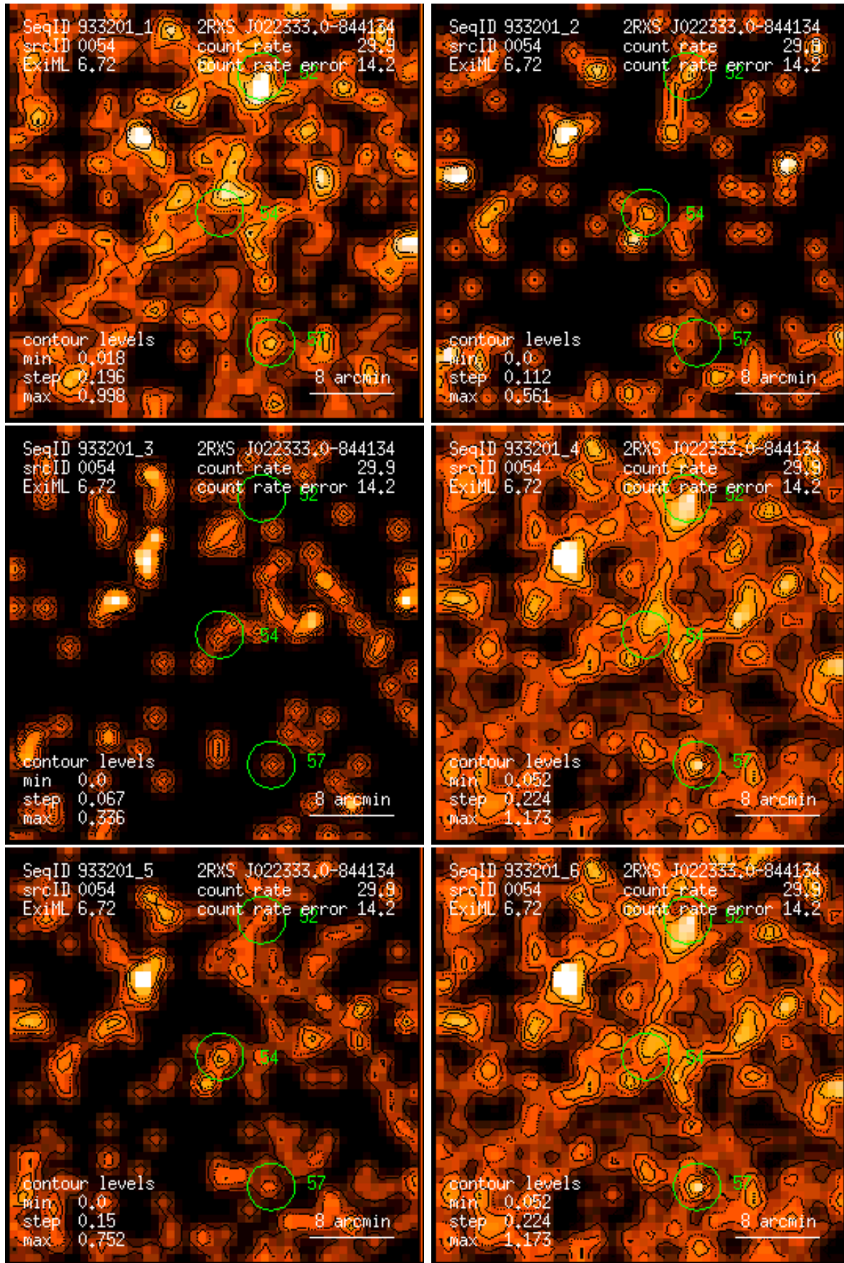
Figure 54: RASS 933201: detection 0054: band rate images, Gaussian filter: (1) PSPC channels 11 – 41, (2) 52 – 90, (3) 91 – 201, (4) 11 – 235, (5) 52 – 201, (6) 11 – 201. Broad band rates in counts/ks. Band rate contour levels in counts/ks/arcmin 2 .
