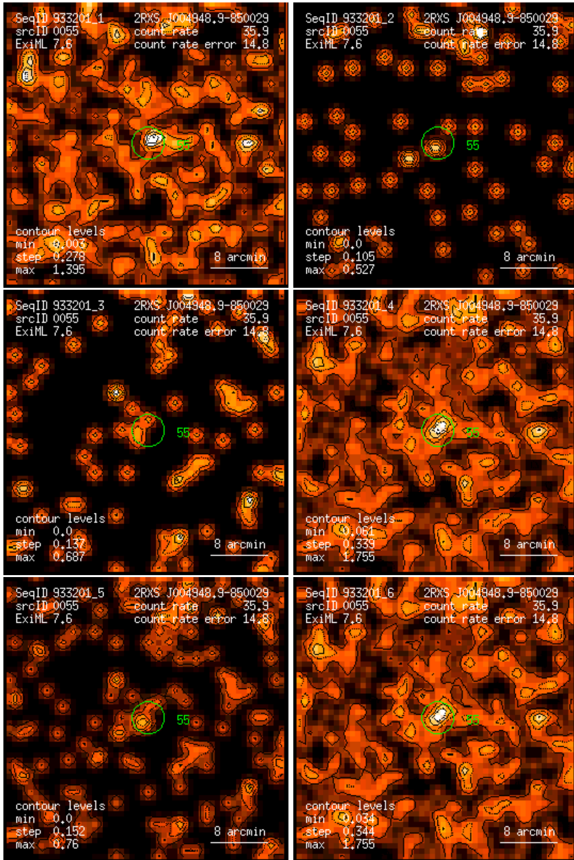
Figure 55: RASS 933201: detection 0055: band rate images, Gaussian filter: (1) PSPC channels 11 – 41, (2) 52 – 90, (3) 91 – 201, (4) 11 – 235, (5) 52 – 201, (6) 11 – 201. Broad band rates in counts/ks. Band rate contour levels in counts/ks/arcmin 2 .
