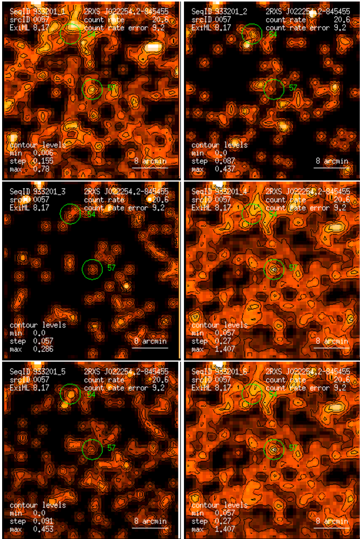
Figure 57: RASS 933201: detection 0057: band rate images, Gaussian filter: (1) PSPC channels 11 – 41, (2) 52 – 90, (3) 91 – 201, (4) 11 – 235, (5) 52 – 201, (6) 11 – 201. Broad band rates in counts/ks. Band rate contour levels in counts/ks/arcmin 2 .
