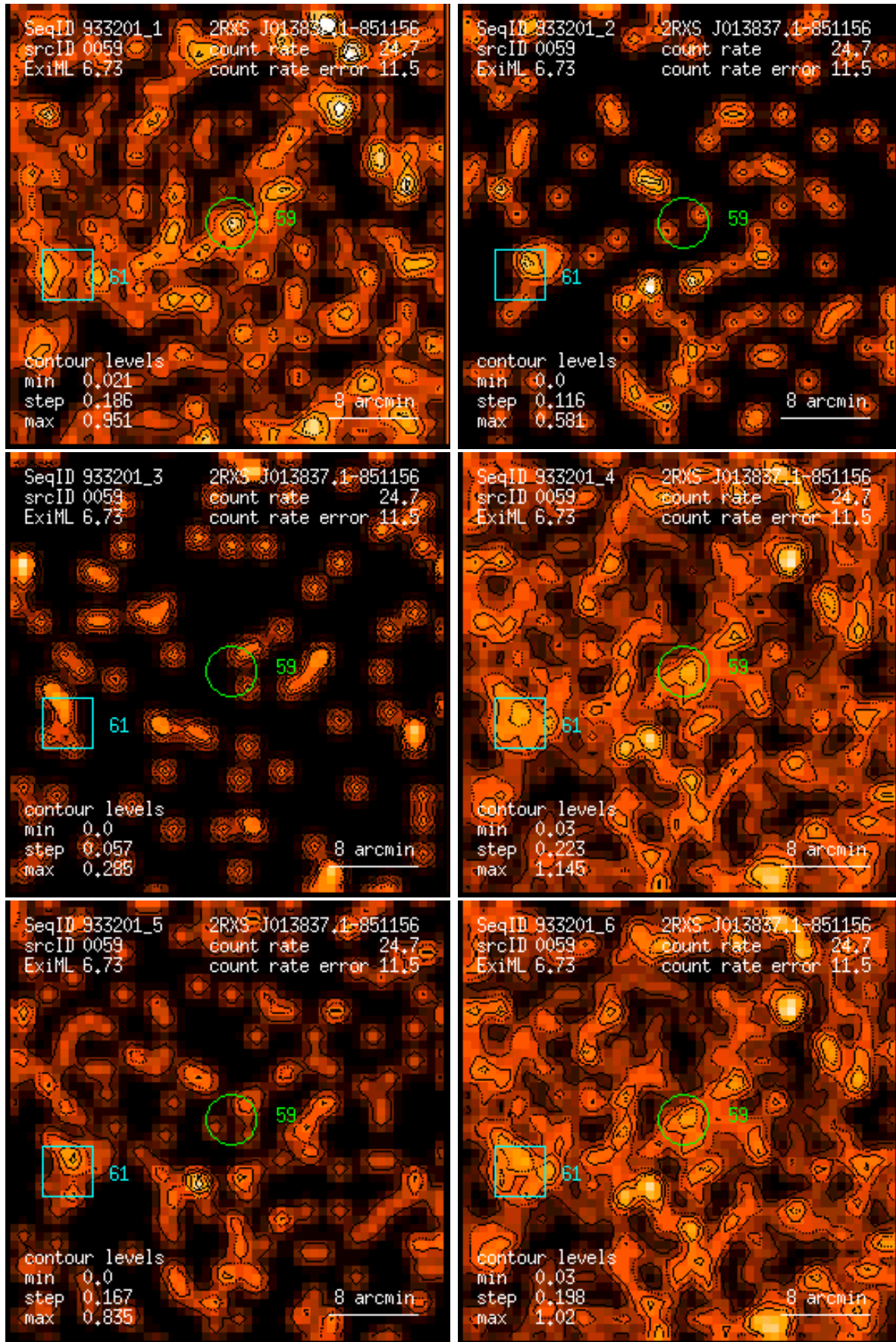
Figure 59: RASS 933201: detection 0059: band rate images, Gaussian filter: (1) PSPC channels 11 – 41, (2) 52 – 90, (3) 91 – 201, (4) 11 – 235, (5) 52 – 201, (6) 11 – 201. Broad band rates in counts/ks. Band rate contour levels in counts/ks/arcmin 2 .
