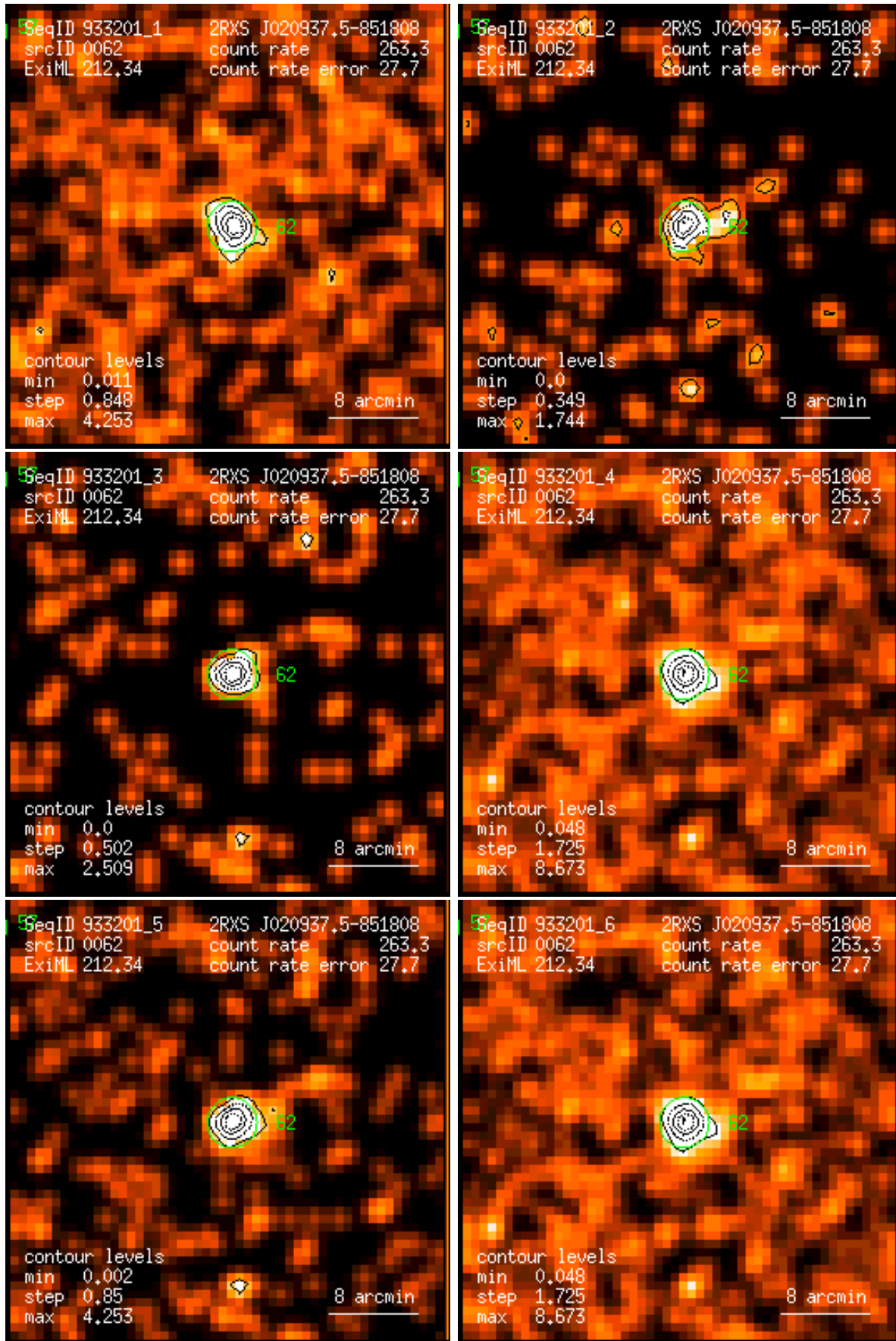
Figure 62: RASS 933201: detection 0062: band rate images, Gaussian filter: (1) PSPC channels 11 – 41, (2) 52 – 90, (3) 91 – 201, (4) 11 – 235, (5) 52 – 201, (6) 11 – 201. Broad band rates in counts/ks. Band rate contour levels in counts/ks/arcmin 2 .
