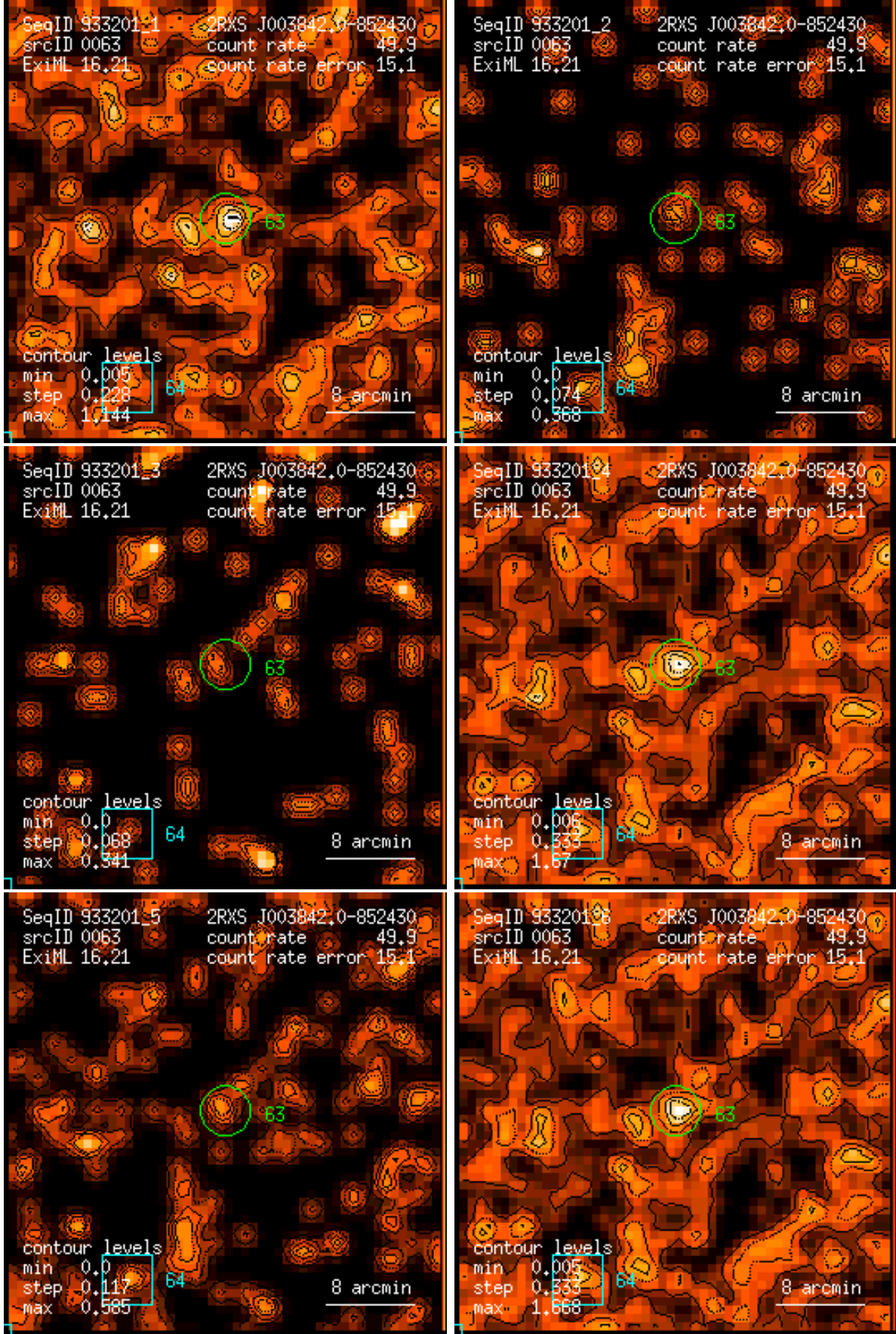
Figure 63: RASS 933201: detection 0063: band rate images, Gaussian filter: (1) PSPC channels 11 – 41, (2) 52 – 90, (3) 91 – 201, (4) 11 – 235, (5) 52 – 201, (6) 11 – 201. Broad band rates in counts/ks. Band rate contour levels in counts/ks/arcmin 2 .
