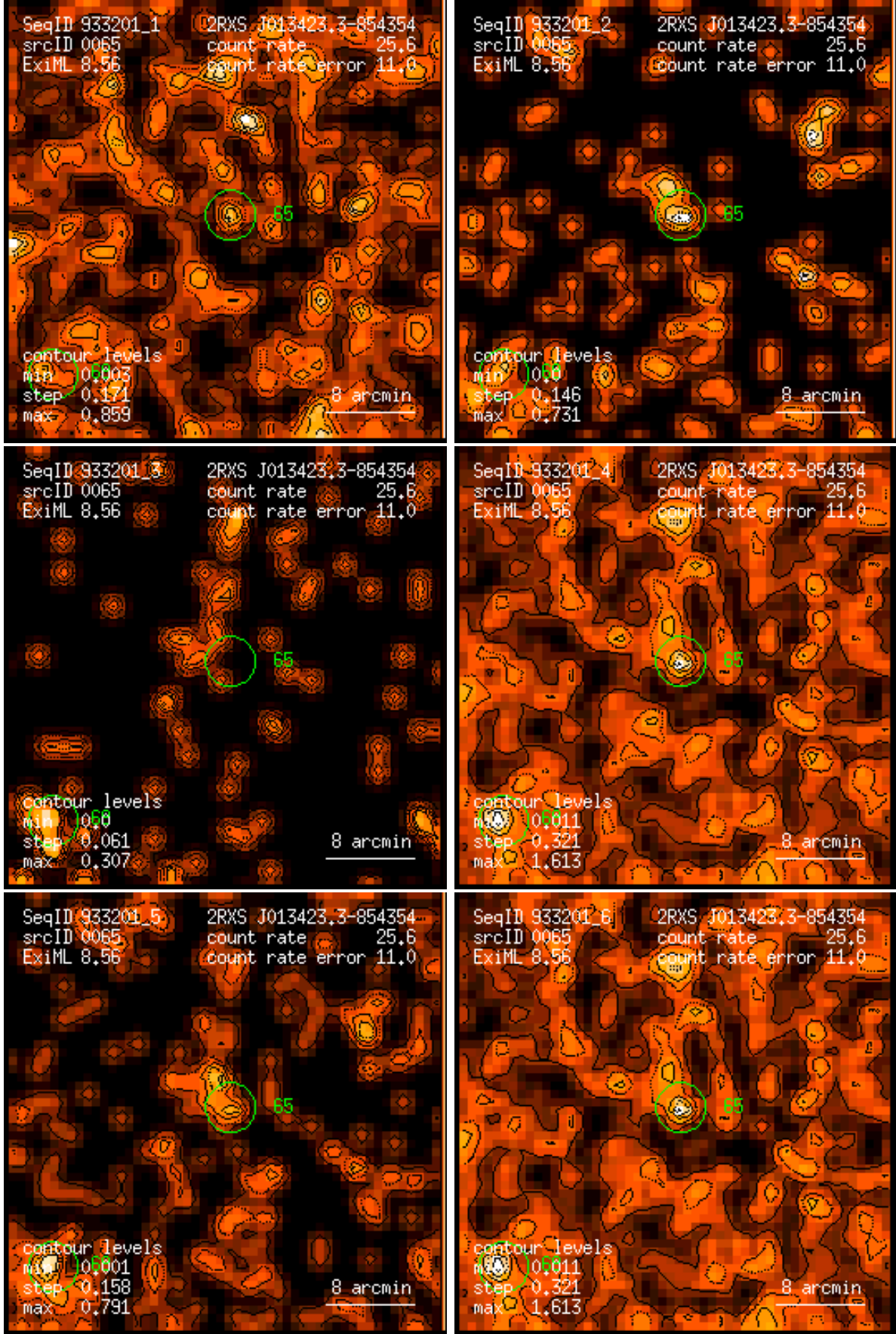
Figure 65: RASS 933201: detection 0065: band rate images, Gaussian filter: (1) PSPC channels 11 – 41, (2) 52 – 90, (3) 91 – 201, (4) 11 – 235, (5) 52 – 201, (6) 11 – 201. Broad band rates in counts/ks. Band rate contour levels in counts/ks/arcmin 2 .
