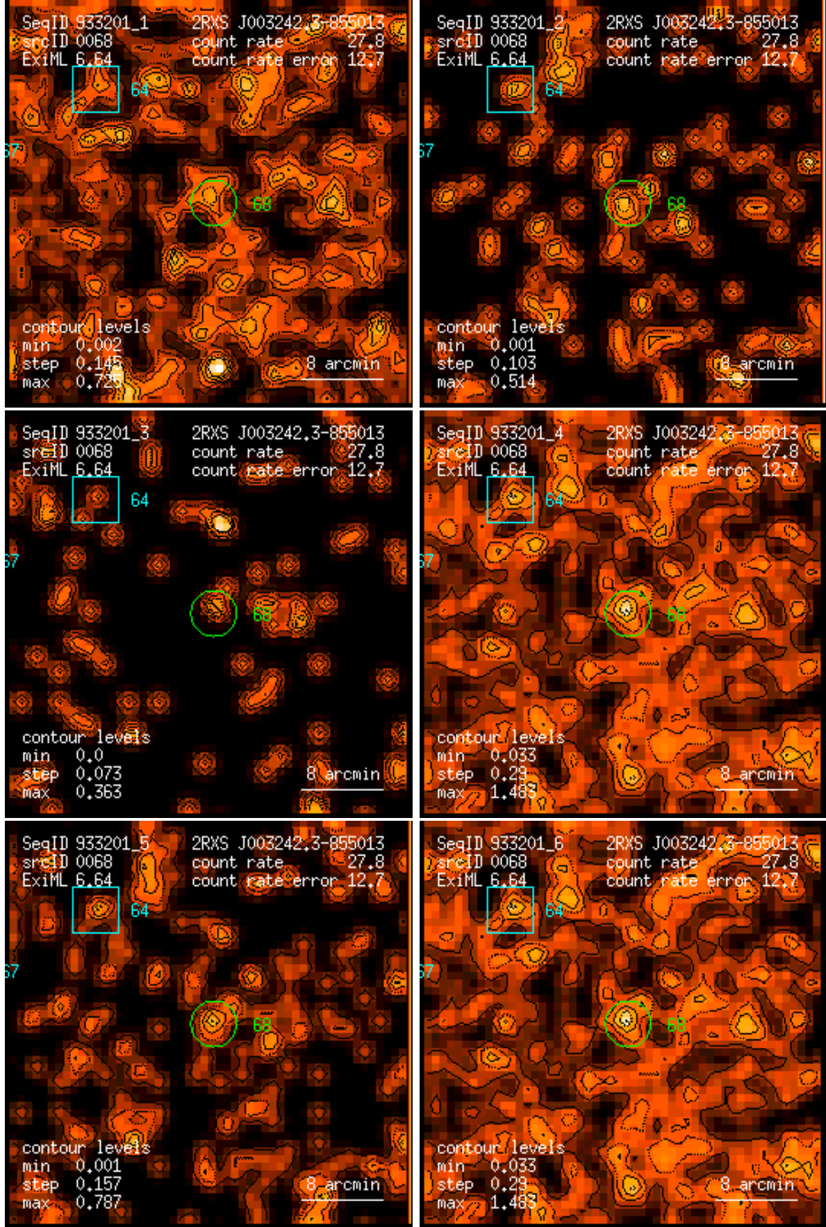
Figure 68: RASS 933201: detection 0068: band rate images, Gaussian filter: (1) PSPC channels 11 – 41, (2) 52 – 90, (3) 91 – 201, (4) 11 – 235, (5) 52 – 201, (6) 11 – 201. Broad band rates in counts/ks. Band rate contour levels in counts/ks/arcmin 2 .
