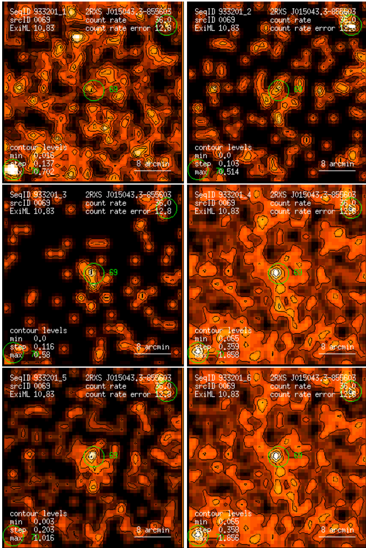
Figure 69: RASS 933201: detection 0069: band rate images, Gaussian filter: (1) PSPC channels 11 – 41, (2) 52 – 90, (3) 91 – 201, (4) 11 – 235, (5) 52 – 201, (6) 11 – 201. Broad band rates in counts/ks. Band rate contour levels in counts/ks/arcmin 2 .
