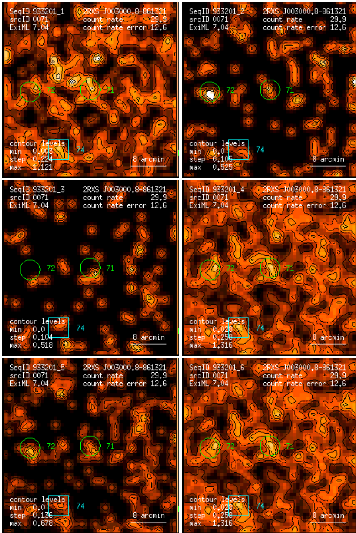
Figure 71: RASS 933201: detection 0071: band rate images, Gaussian filter: (1) PSPC channels 11 – 41, (2) 52 – 90, (3) 91 – 201, (4) 11 – 235, (5) 52 – 201, (6) 11 – 201. Broad band rates in counts/ks. Band rate contour levels in counts/ks/arcmin 2 .
