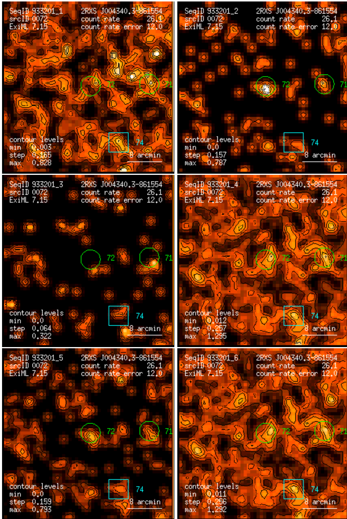
Figure 72: RASS 933201: detection 0072: band rate images, Gaussian filter: (1) PSPC channels 11 – 41, (2) 52 – 90, (3) 91 – 201, (4) 11 – 235, (5) 52 – 201, (6) 11 – 201. Broad band rates in counts/ks. Band rate contour levels in counts/ks/arcmin 2 .
