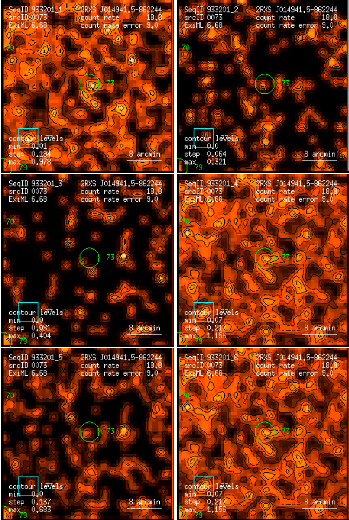
Figure 73: RASS 933201: detection 0073: band rate images, Gaussian filter: (1) PSPC channels 11 – 41, (2) 52 – 90, (3) 91 – 201, (4) 11 – 235, (5) 52 – 201, (6) 11 – 201. Broad band rates in counts/ks. Band rate contour levels in counts/ks/arcmin 2 .
