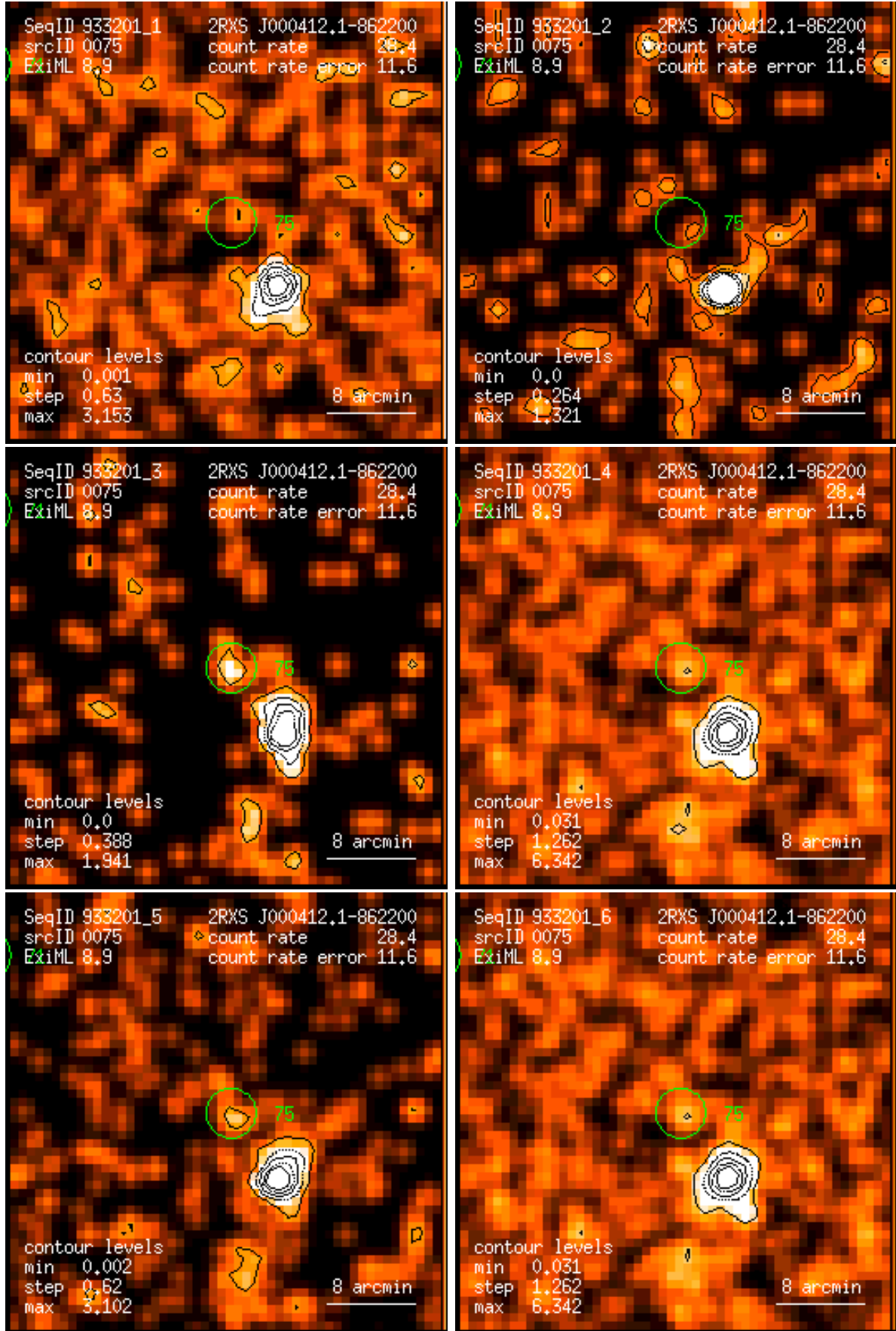
Figure 75: RASS 933201: detection 0075: band rate images, Gaussian filter: (1) PSPC channels 11 – 41, (2) 52 – 90, (3) 91 – 201, (4) 11 – 235, (5) 52 – 201, (6) 11 – 201. Broad band rates in counts/ks. Band rate contour levels in counts/ks/arcmin 2 .
