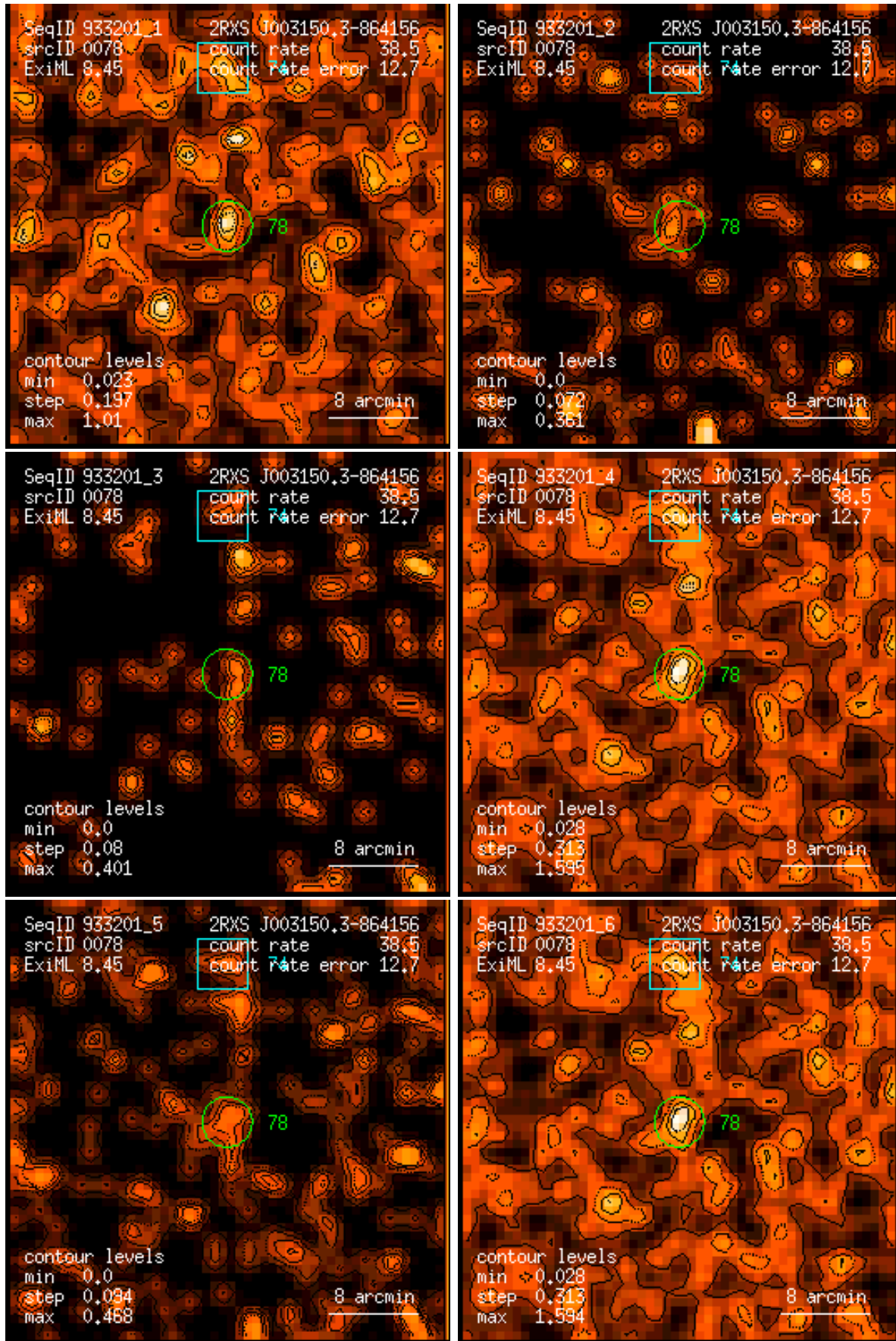
Figure 78: RASS 933201: detection 0078: band rate images, Gaussian filter: (1) PSPC channels 11 – 41, (2) 52 – 90, (3) 91 – 201, (4) 11 – 235, (5) 52 – 201, (6) 11 – 201. Broad band rates in counts/ks. Band rate contour levels in counts/ks/arcmin 2 .
