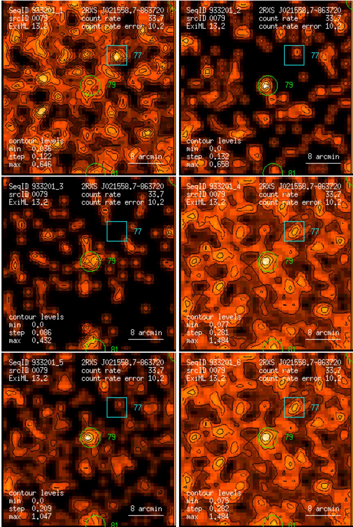
Figure 79: RASS 933201: detection 0079: band rate images, Gaussian filter: (1) PSPC channels 11 – 41, (2) 52 – 90, (3) 91 – 201, (4) 11 – 235, (5) 52 – 201, (6) 11 – 201. Broad band rates in counts/ks. Band rate contour levels in counts/ks/arcmin 2 .
