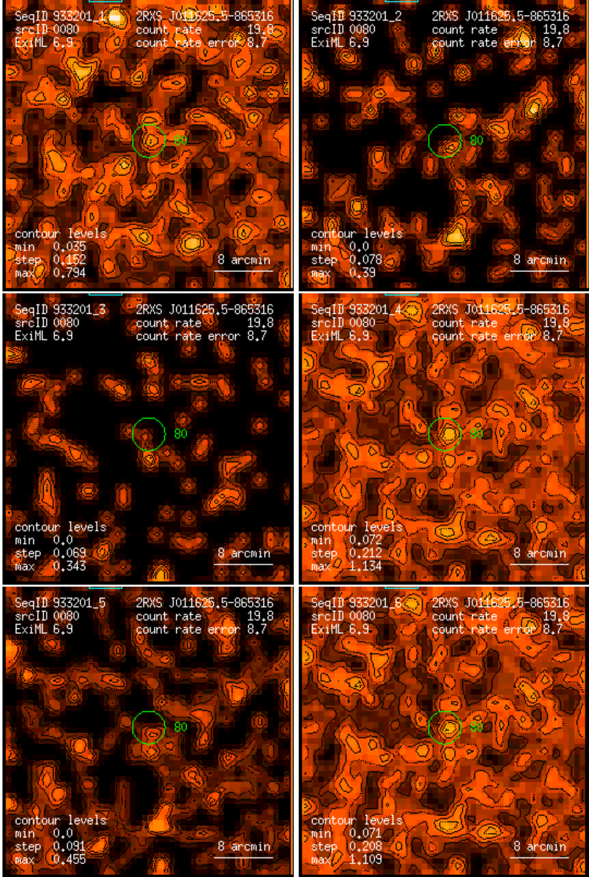
Figure 80: RASS 933201: detection 0080: band rate images, Gaussian filter: (1) PSPC channels 11 – 41, (2) 52 – 90, (3) 91 – 201, (4) 11 – 235, (5) 52 – 201, (6) 11 – 201. Broad band rates in counts/ks. Band rate contour levels in counts/ks/arcmin 2 .
